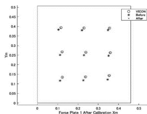
Fig. 2. Position of COP_v and COP_f data of the force plate 1 after calibration.
