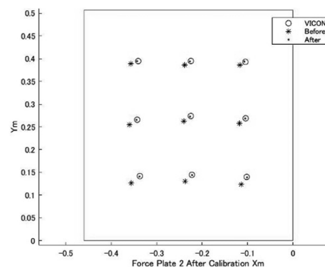
Fig. 3. Position of COP_v and COP_f data of the force plate 2 after calibration.
