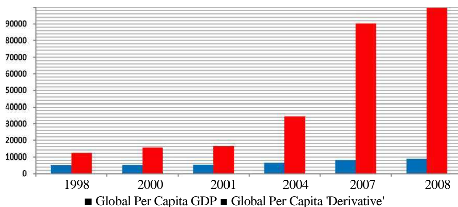
Figure 1: World Per Capita Derivative and Per Capita GDP 1000
