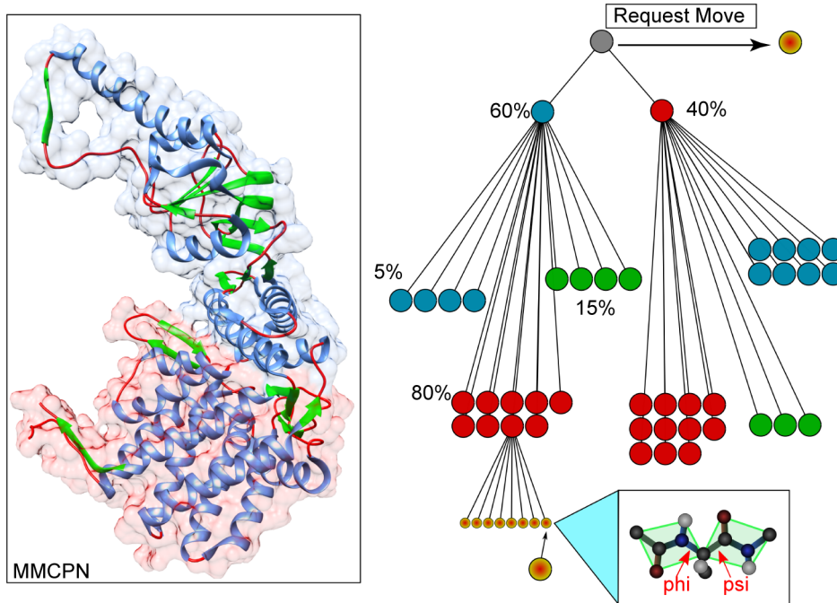
Figure 1. Example of a structured schema for an arbitrary molecule. Subsets of DOFs are defined, along with the associated weighting (shown here as percentages) defining the relative probability of selection. Though this example is non-overlapping and hierarchical, any combination of possibly non-contiguous subsets are allowed in our implementation. In this example, a move is generically requested, and subsequently sampled probabilistically from the set containing all loop regions in the top (blue) region of the structure. The yellow circles represent possible moves. doi:10.1371/journal.pone.0068826.g001
