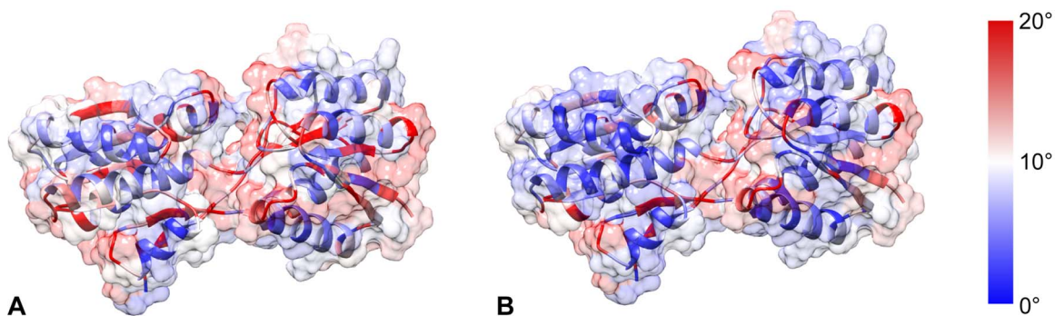
Figure 5. Plot of active DOFs for expert (A) and auto (B) experiments. Color bar indicates cumulative per-residue torsional change over the entire determined transition. The two experiments show comparable activity in torsional DOFs, largely confined to central loops through which much of the bending occurs. doi:10.1371/journal.pone.0068826.g005
