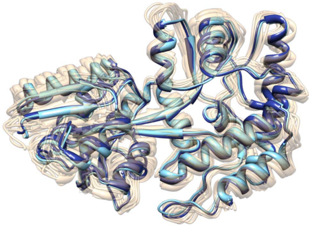
Figure 8. Comparison of a computationally identified intermediate state and NMR structure PDB:2H25. The identified intermediate state (dark blue) corresponds to the centroid of the low energy region shown in Figure 7. The NMR structure is known to be close to the semi-closed conformation of MBP, showing excellent agreement at the resolution of the ensemble. The closest state along a direct transition between known open and bound forms (aqua structure) of MBP to PDB:2H25 shows almost perfect agreement with the centroid structure. doi:10.1371/journal.pone.0068826.g008
