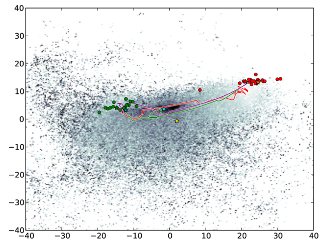
Figure 7. pca landscape of all conformations generated in the MBP experiments. Each point represents a unique conformation. The color indicates energy with darker colors representing more energetically stable states. The red path shows the path found with the default schema, starting from the open state with the bound state as the goal. The green path represents the reverse case, with the default schema, starting at the bound state and moving toward the open state. The purple path was produced using the expert- schema, moving from the bound state towards the open state. The yellow star indicates the position of a known NMR structure (PDB:2H25) of the semi-closed state. The aqua star indicates the centroid conformation of the energetic valley between the open and bound states and falls extremely close to all paths, as well as the NMR structure. The circular pattern in the green path was automatically generated and seems to arise from a slight bending reversal that occurs near the semi-closed state. doi:10.1371/journal.pone.0068826.g007
