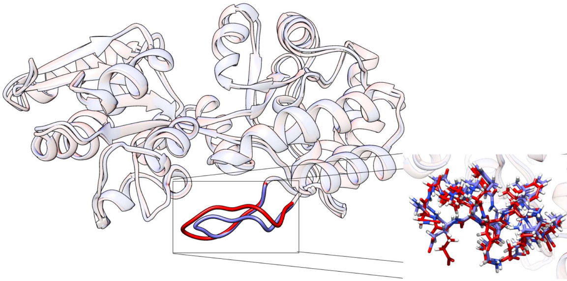
Figure 6. Comparison of the final state of the reverse transition (blue) and the direct transition (red). Structures are nearly identical save for a 10 residue relaxation of a loop region in the balancing interface. Both transitions come to within 1Å of their goal. doi:10.1371/journal.pone.0068826.g006
