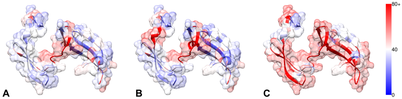
Figure 3. Plots of angular change in DOFs for hinge (A), hinge+flex (B) and auto (C) experiments. Residues are colored by absolute total angular change, with blue indicating a small change and red a large change. Hinge and Flex (A, B) experiments show relatively low activity outside of the planning regions. The automatically guided experiment (C) shows high activity in the hinge and \beta -sheet regions of both subdomains. doi:10.1371/journal.pone.0068826.g003
