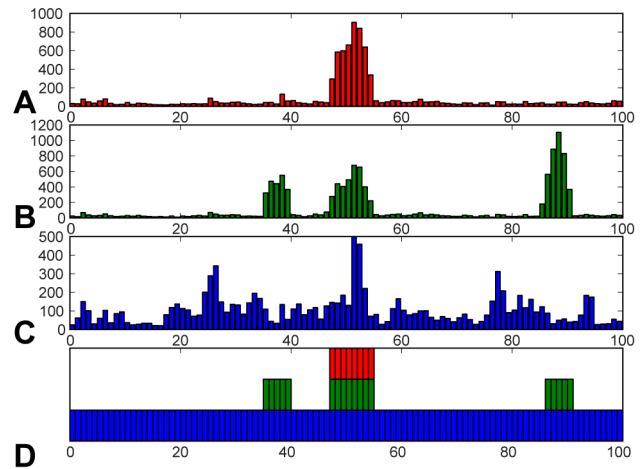
Figure 2. Plots of total angular change for each residue over the determined transition. (A) Central hinge only. (B) Hinge+flex region. (C) Automatic. (D) shows active residues explicitly used in planning for hinge (red), hinge+flex (green) and automatic (blue) runs. doi:10.1371/journal.pone.0068826.g002
