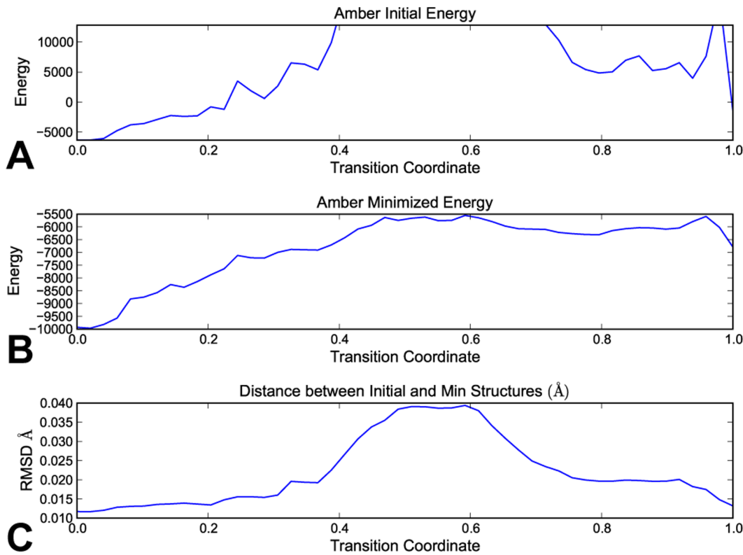
Figure 4. Energies as calculated by the Amber99 forcefield for a typical automatically guided run. All experiments produced similar plots. Energies are plotted against the transition coordinate (the amount of progress between start and goal for the transition). (A) Amber energies for the raw output of the automatically guided run (B) Amber energies after 100 rounds of minimization (C) Distance between raw output and minimized structure. All structures are determined to be of low energy, post-minimization, according to the Amber forcefield, with only mild (much less than 0.1Å full-atom \text{RMSD} ) differences between the two structures. doi:10.1371/journal.pone.0068826.g004
