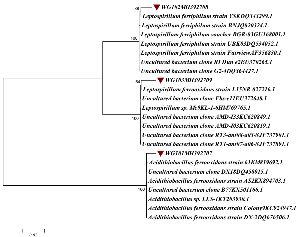
Fig. 1 Molecular phylogenetic analysis of indigenous iron-oxidizing bacteria by maximum likelihood method based on homologues sequences obtained from GenBank database. The tree with the highest log likelihood (−3431.6230) is shown. The analysis involved 24 nucleotide sequences. Codon positions included were 1st + 2nd + 3rd + noncoding. Evolutionary analyses were conducted in
