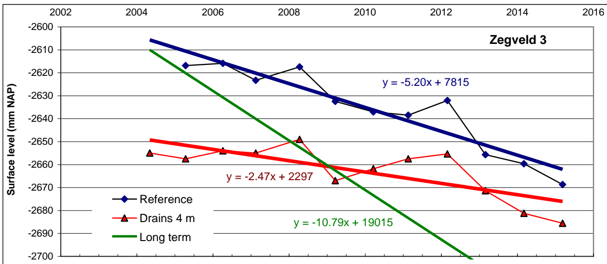
Fig. 2: Subsidence 2004 – 2015 of peat soil without submerged drains (Reference) and with submerged drains at a distance of 4 meters (Drains 4 m). The long term subsidence is 10.8 mm per year. NAP = the Dutch national reference level, which is about the average sea water level.
