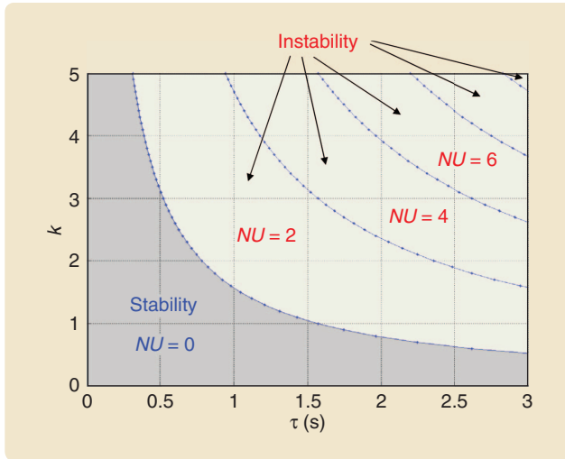
FIGURE 8 Stability chart with respect to the delay \tau and controller gain k . The plot depicts the stability chart of a closed-loop system with the transfer function H(s) = 1/s and the control law C(s) = -ke^{-\tau s} , where 0 \leq k \leq 5 . Each pair (\tau, k) selected from the shaded region leads to stability of the control system. If, for a given pair (\tau, k) , the system is stable, then the number NU of unstable roots is zero.
