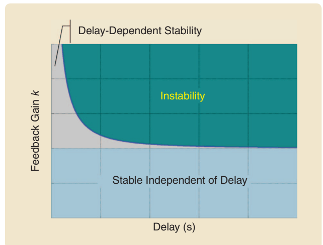
FIGURE 4 Stability chart. This chart is obtained for a closed-loop system with the plant transfer function e^{-\tau s}b/(s + a) and the controller C(s) = k . This stability chart is partitioned into three regions, namely, delay-independent stable, delay-dependent stable, and unstable. This chart reveals the effect of a delay parameter on stability and how the controller gain k can be tuned to avoid instability.
