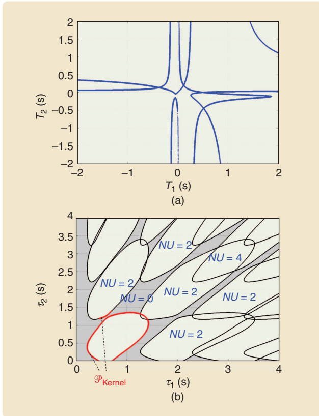
FIGURE 21 Mapping from the parametric domain (T_1, T_2) to the delay domain (\tau_1, \tau_2) . The domain (T_1, T_2) in (a) is used to detect the stability-switching curves (SSCs) in the delay domain in (b). These curves are essential for stability analysis since they determine the boundaries that separate stability from instability in the delay domain. To find SSCs, the points (T_1, T_2) that create imaginary roots s = j\omega in (54) are crucial. In (a), these points are depicted for this numerical example. Next, using the triplets (\omega, T_1, T_2) , SSCs can be obtained from (53) as shown in (b). In (b), the stability regions in the delay domain are shaded, the number NU of unstable roots is shown, and the kernel curve is marked. In this stability analysis, we see that multiple disjoint stability regions arise, offering several choices to select or schedule the delays in the closed-loop system in order to stabilize the system.
