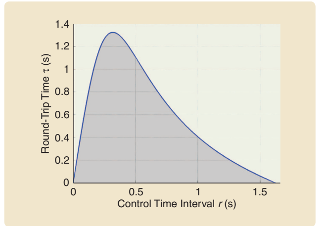
FIGURE 20 Stability chart. The shaded regions in the delay-parameter space (\tau, r) represent the stability regions of the congestion control model (50). The delay r \neq 0 , which is the control-time interval, can be chosen to guarantee stability for a round-trip time as large as \tau \approx 1.3 s.
