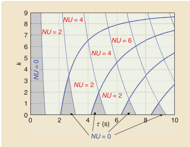
FIGURE 10 Stability chart with respect to the delay \tau and controller gain k . This plot depicts the stability chart of a closed-loop control system with the transfer function H(s) = 1/(s^2 + \omega_0^2) and the control law C(s) = ke^{-\tau s} , where \omega_0 = 3 and 0 < k < 9 . Each pair (\tau, k) selected from the shaded regions leads to stability of the control system, that is, the number NU of unstable roots is zero.
