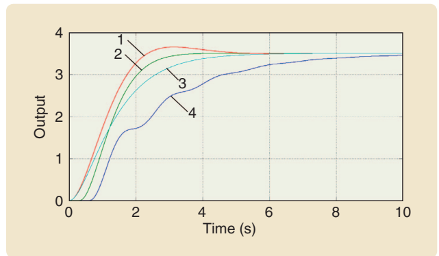
FIGURE 11 Step response. The positive feedback control loop consists of the open-loop transfer function H(s) = 1/(s^2 + 9) and the controller C(s) = (k_p e^{-\tau s} + k_d s) . The aim is to compare the speed of response between a delay-free proportional-derivative controller ( k_p \neq 0, k_d \neq 0, \tau = 0 ) and a delayed proportional controller ( k = k_p \neq 0, \tau \neq 0 , and k_d = 0 ). Curve 1 denotes the case where there is no delay in the closed-loop system with the controller gains k_p = 7 and k_d = -2 . Curve 2 corresponds to the output of the system with \tau = 0.3 s and the proportional controller gain k = 7 . Curve 3 represents the output of the system with no delay and controller gains k_p = 7 and k_d = -3 . Finally, curve 4 denotes the output of the system with delay \tau = 0.6 s and controller gain k = 7 .
