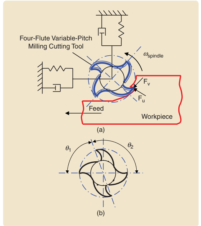
FIGURE 5 Variable-pitch milling. A four-flute cutting tool with pitch angles \theta_1 and \theta_2 is used to machine a metal workpiece. Due to the flexibility of the tool, each tooth leaves some uncut material, which is encountered by the next tooth as an additional force. That is, a past event affects the evolution of the cutting dynamics. The delays that arise from this mechanism are proportional to the tooth-passing period.
