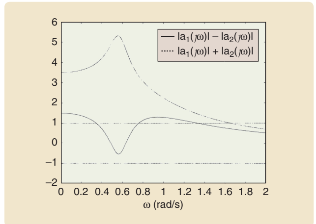
FIGURE 15 Frequency-sweeping test. By sweeping the frequency \omega , the norm |a_1(j\omega)| \pm |a_2(j\omega)| is visualized as a function of \omega for the system (46) and (47). This plot yields the range of frequencies for which the triangle conditions (44)–(45) hold. These frequency ranges generate the delay solutions \tau_1 - \tau_2 in figures 16 and 17. (Reprinted from [92] with permission from Elsevier.)
