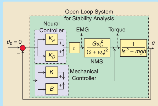
FIGURE S3 Control diagram for quiet standing. The experimental setup in Figure S2 and its control structure are depicted in this block diagram. An active correction mechanism, which is typically considered as a proportional-derivative controller, emanates from the neural controller and becomes effective after a length of time \tau . The neuromusculoskeletal system models the response of the muscles with critically damped second-order dynamics whose natural frequency is \omega_n . The human body, which is modeled as an inverted pendulum with inertia I , mass m , and center of mass at height h , responds to the torques originating from the neuromusculoskeletal system and the mechanical controller representing the mechanics of muscles. The electromyography signals shown here are measured at the ankles. (Used with permission of APS. See [19] for full citation information.)
