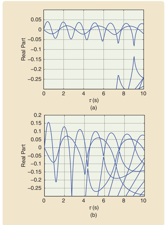
FIGURE 13 Rightmost root distributions of (24). The curves in (a) and (b) show how the real part of the rightmost roots of the characteristic equation (24) vary with respect to the delay \tau , where \omega_1 = 2 and \omega_2 = 4 . (a) and (b) correspond to \varepsilon = 1/4 and \varepsilon = 1 in the numerical example, respectively.
