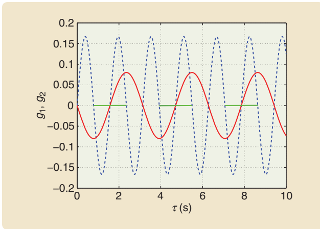
FIGURE 12 Verification of stable poles. Using the sinusoidal functions in (25), the location of the poles in the complex plane can be determined. The sign agreement between g_1 and g_2 indicates that the closed-loop system is stable. This example shows that stability can be deduced from the phase synchronization of two functions g_1 and g_2 , derived from the characteristic equation of the system.
