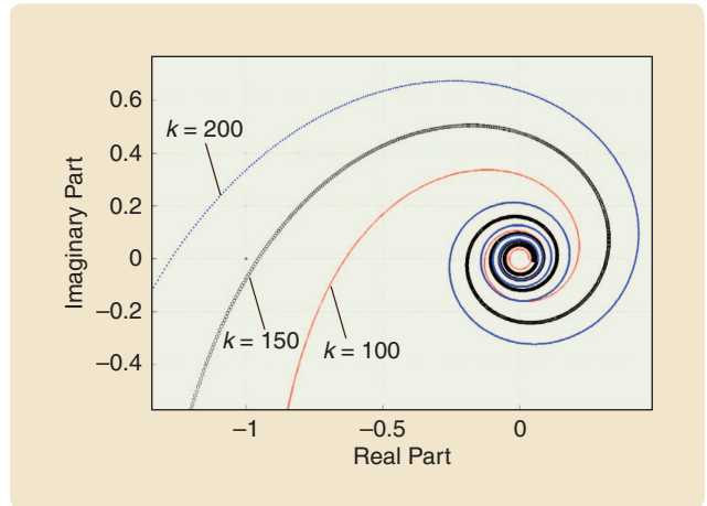
FIGURE 7 Nyquist plot for several controller gains k . The closed-loop control system consists of the transfer function H(s) = 1/s and the proportional feedback control law C(s) = -ke^{-s\tau} with delay \tau = 0.01 s.
