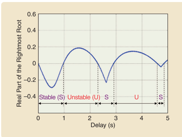
FIGURE 9 Behavior of the real part of the rightmost root. For a closed-loop system with the characteristic equation f(s; \tau) = s^2 + 9 - 1.5e^{-\tau s} = 0 , this plot depicts how the real part of the rightmost characteristic root behaves with respect to the delay parameter \tau . The sign change of the real part indicates that the closed-loop system switches from stability to instability several times.
