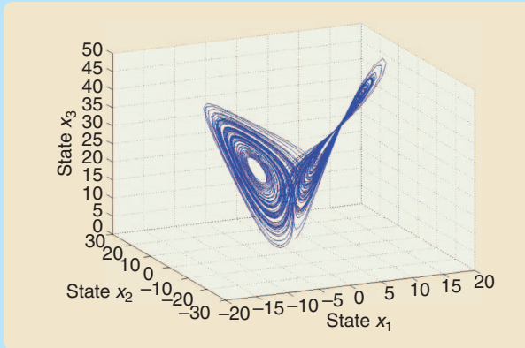
FIGURE S8 The Lorenz attractor. This attractor, which is in \mathbb{R}^3 , is composed of an infinite number of unstable limit cycles. For the particular choice of the parameters in Example 9, all trajectories converge to the chaotic attractor. This attractor illustrates both the long-term unpredictability and boundedness of the trajectories.
