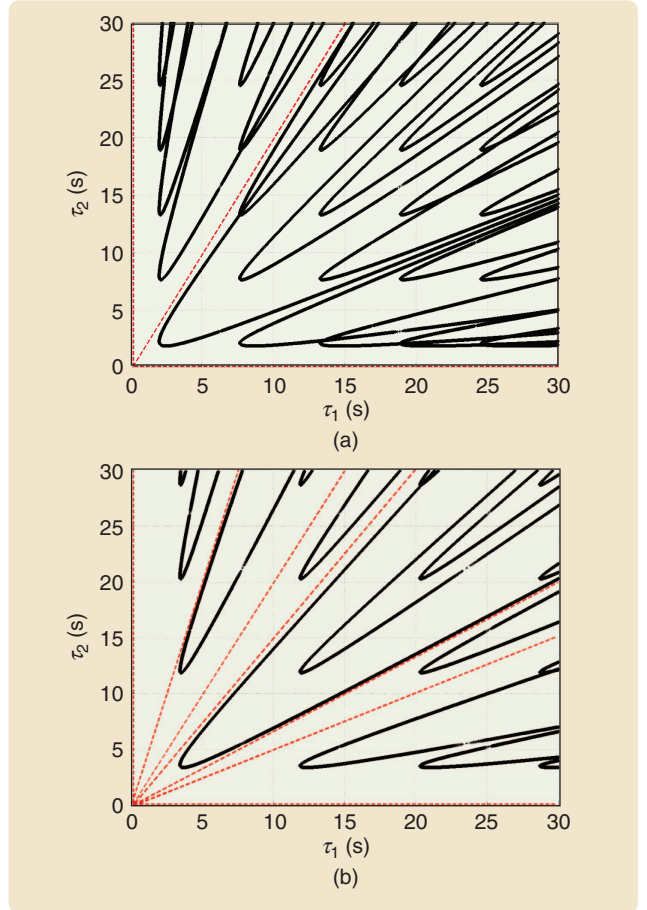
FIGURE 23 Investigation of delay interference. Stability and instability regions of (59) are presented in the (\tau_1, \tau_2) -space for a = 1 (left) and a = 1.3 (right). For a = 1 , three stable rays, two of which are the axes, exist. If a = 1.3 , then the number of rays including the axes is seven. These rays, which are shown with dashed lines, define all combinations of multiple delays for which the closed-loop system remains stable. That is, the system is stable independently of the delays that lie on these rays. When constructing controllers, the existence of such rays can be useful, but instability can occur when the slopes of these rays are perturbed due to uncertainty in the delays.
