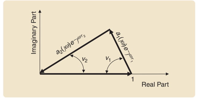
FIGURE 14 Geometric interpretation of (43). Equation (43) is represented in the complex plane as the sum of three vectors. If these vectors create a triangle in the complex domain, then the characteristic equation has a solution at s=j\omega for some delays \tau_1 and \tau_2 . For all delay values, since the norms of the vectors are independent of the delays, we can write conditions, called triangle inequalities , for a triangle to form on the complex plane. These conditions, which involve only \omega , are based on the fact that the length of each edge of a triangle cannot exceed the sum of the lengths of the remaining two edges. Once all \omega satisfying these triangle conditions are determined, the delays \tau_1 and \tau_2 can be calculated using \omega and the orientation of the vectors.
