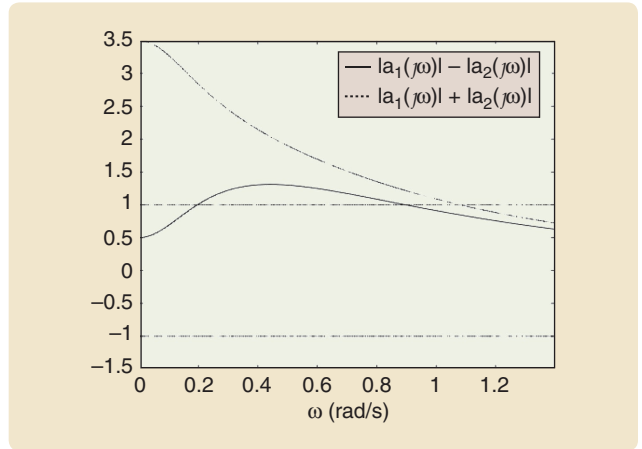
FIGURE 18 Frequency-sweeping test. By sweeping the frequency \omega , the norm |a_1(j\omega)| \pm |a_2(j\omega)| is visualized as a function of \omega for the system (48) and (49). This plot yields the range of frequencies for which the triangle conditions (44), (45) hold. These frequency ranges generate the delay solutions \tau_1 - \tau_2 in Figure 19. (Reprinted from [92] with permission from Elsevier.)
