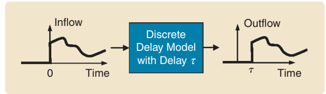
FIGURE 3 Constant delay model. Delay can be modeled as a buffer that holds the inflow signal for a length of time and then releases the signal without distortion. This type of delay represents a first-in, first-out-type model found in sensing, information transmission, and mass transport.
