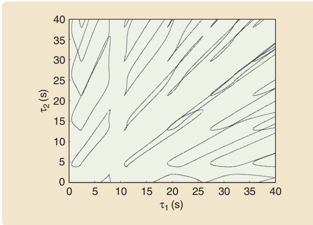
FIGURE 16 Delay solutions on closed curves. The curves C_1 of the system in Example 6 are the stability-switching curves, which represent the delay values for which the characteristic equation has a pair of roots on the imaginary axis. These curves decompose the delay plane into regions in which all delays lead to the same number NU of unstable roots of the system. (Reprinted from [92] with permission from Elsevier.)
