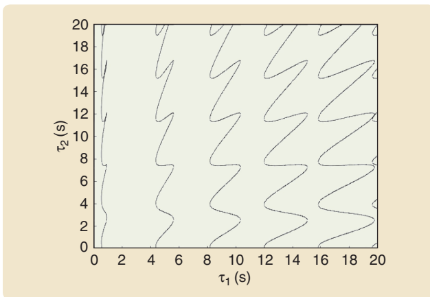
FIGURE 17 Delay solutions on open-ended spirals. The curves C_2 of the system in Example 6 are the stability-switching curves, which represent the delay values with which the characteristic equation has a pair of roots on the imaginary axis. These curves decompose the delay plane into regions in which all delays lead to the same number NU of unstable roots. (Reprinted from [92] with permission from Elsevier.)
