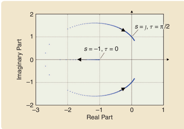
FIGURE 6 Rightmost characteristic roots on the complex plane. This plot shows the location of the rightmost characteristic roots of the closed-loop system with the characteristic equation s + ke^{-s\tau} = 0 for various values of \tau \in [0, 2] with k = 1 . For \tau = \pi/(2k) , the rightmost root crosses toward the right-half plane causing instability. The rightmost roots are computed using DDE-BIFTOOL, which is a numerical bifurcation tool developed for delay differential equations [80].
