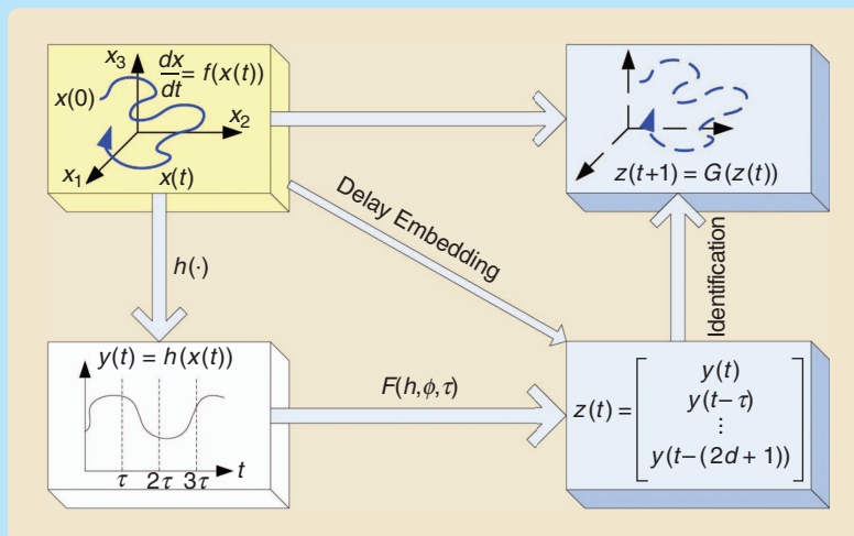
FIGURE S7 The embedding and prediction algorithms. The mapping F(h, \phi, \tau) provides a delay embedding to reconstruct the vector z(t) , which can then be used to identify the mapping G and predict z(t+1) . Note that the first entry of z(t) is the output y(t) .
