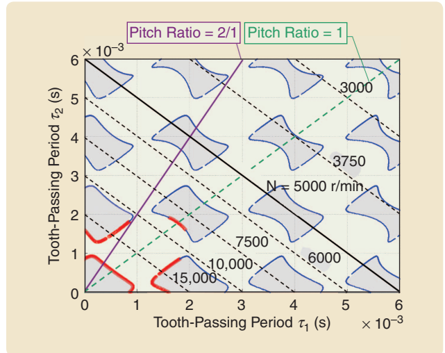
FIGURE 22 Stability chart of the metal-cutting dynamics. The gray shaded regions show the parametric selections corresponding to stability, which refers to machining with vibration-free engagement of the cutting tool with the workpiece. The ratio \tau_2/\tau_1 corresponds to the pitch ratio of the cutting tool, while the lines with slopes -1 correspond to the rotational speed of the spindle in revolutions per minute, which can be chosen appropriately to render stable cutting dynamics, thereby avoiding undesirable vibration at the interface between the cutting tool and the workpiece.
