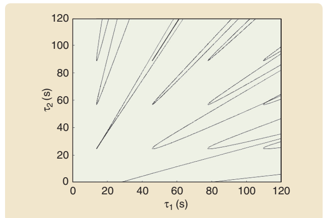
FIGURE 19 Delay solutions on open-ended curves. The delay pairs in the \tau_1 - \tau_2 plane lead to either stability or instability. The boundaries separating the stability and instability regions are determined by the stability-switching curves of the system. In the example (48), (49), these curves are in the form of open-ended forms. (Reprinted from [92] with permission from Elsevier.)
