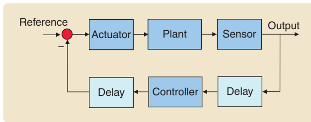
FIGURE 1 Delays in a feedback system. Feedback control systems often function in the presence of delays, primarily due to the time it takes to acquire the information needed for decision-making, to create the control decisions, and to execute these decisions.
