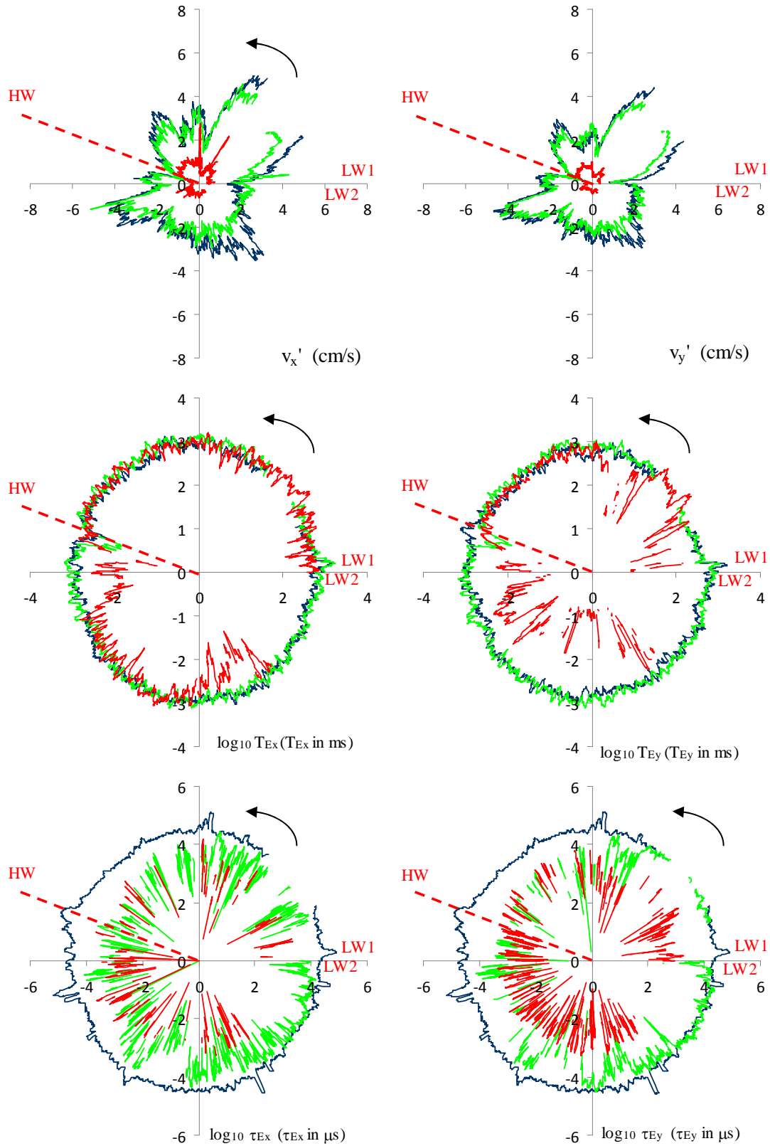
Fig. 10 - Standard deviations of longitudinal and transverse velocity components v_x' and v_y' , integral turbulent time scales T_{Ex} and T_{Ey} , and turbulent dissipation time scales \tau_{Ex} and \tau_{Ey} during a tidal cycle ( t = 197,500 to 217,800 s) - Dark Blue: 0.12 m above bed at Site 2B, Bright Green: 0.32 m above bed at Site 2B, Red: 0.235 m above bed at Site 3
