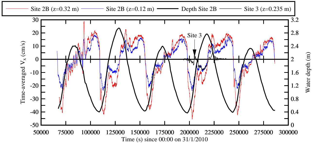
Fig. 4 - Water depth, time-averaged velocity components, time-averaged backscatter intensity and turbidity as functions of time - Data collected at Sites 2B and 3, Eprapah Creek during the study E11 (31 Jun.-3 February 2010) - VITA calculations using the average of the next 10,000 samples (200 s) at 10 s intervals along entire data sets
