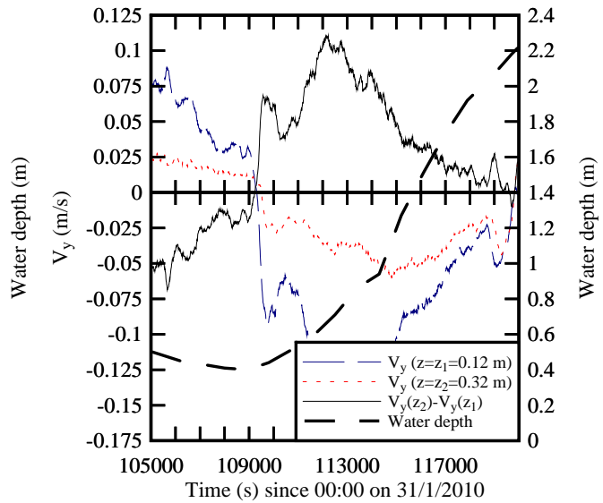
(B) Flood tide on 1 February 2010
