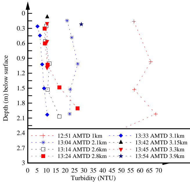
(C1) Turbidity during the early ebb tide
