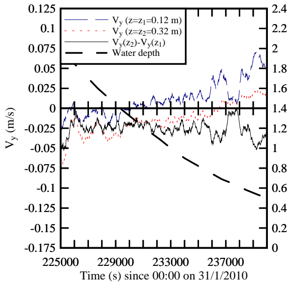
(A) Mid ebb tide on 2 February 2010
