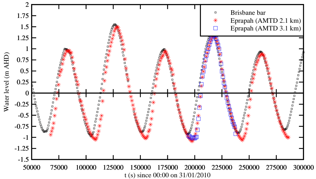
Fig. 2 - Measured water depths at Eprapah Creek on 31 January, 1, 2 and 3 February 2010 - Time since 00:00 on 31 January 2010 - Comparison with the measured water depths at Brisbane bar (Courtesy of Tidal Unit Maritime Safety Queensland - Brisbane)
