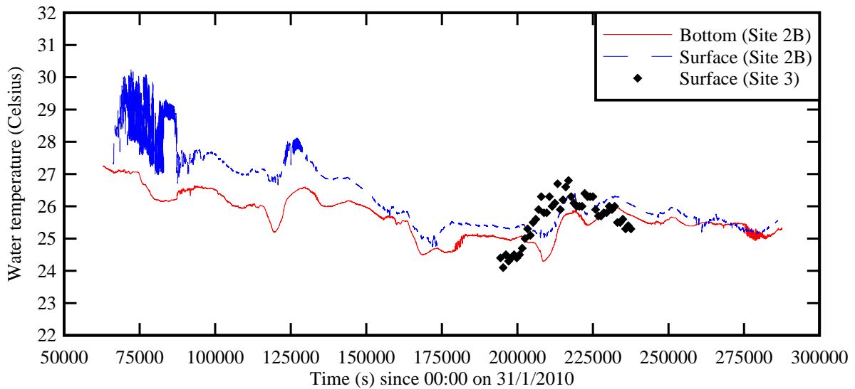
(B) Bottom and surface water temperatures at Sites 2B and 3
