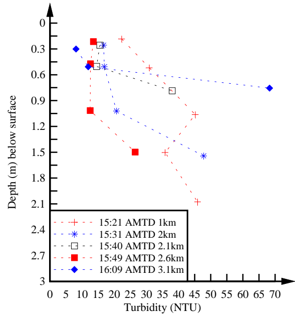
(C2) Turbidity during the mid ebb tide
