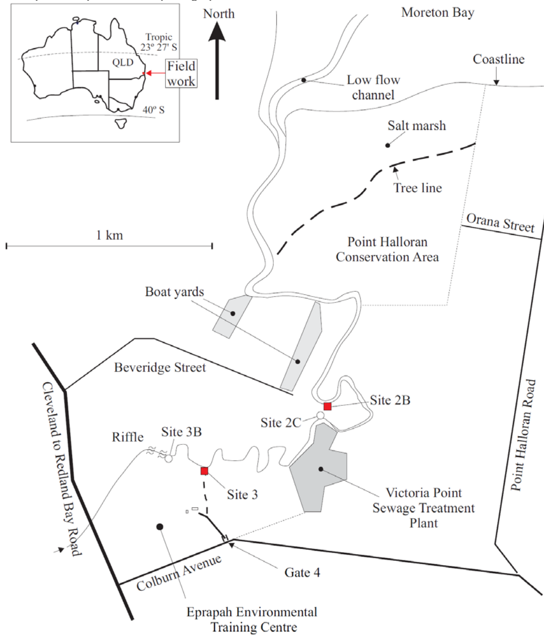
Fig. 1 - Estuarine zone of Eprapah Creek, Australia
