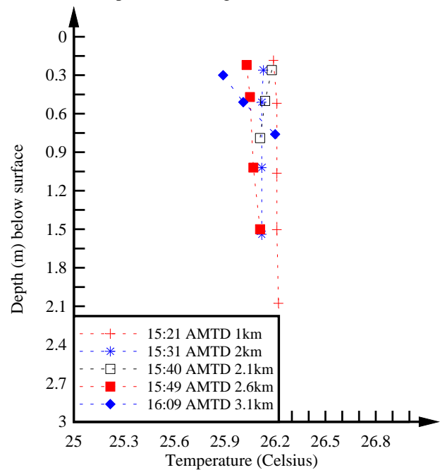
(B2) Water temperature during the mid ebb tide
