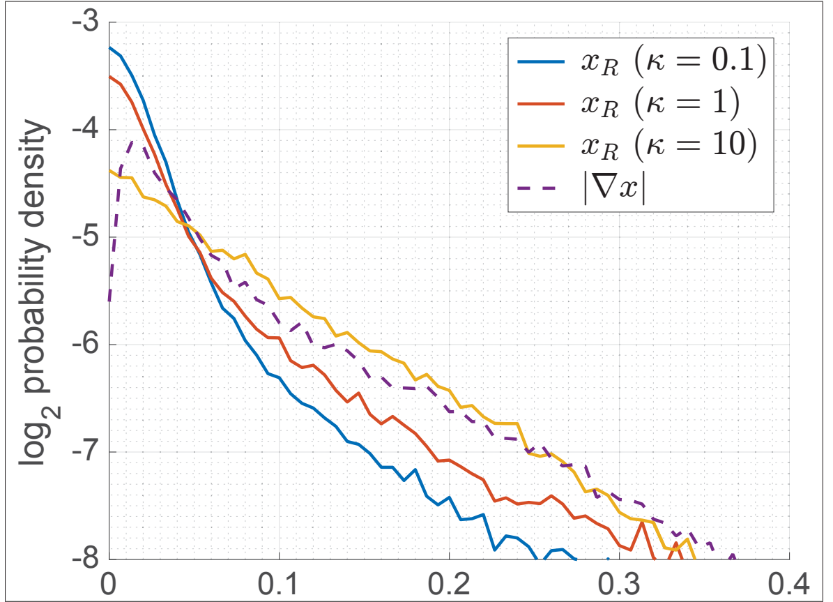
Figure 3.2 Distribution of absolute values in the gradient magnitude and the proposed residual component for different \kappa . Values are shown for the image of Fig. 3.1.
