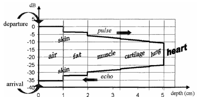
Fig. 2. Model predicted attenuation of pulse-echo intensity traveling from the transmitting antenna to the receiving antenna. Each step accounts for echo at the boundary. Decreasing of the curve accounts for linear attenuation in the tissue (imaginary part of reflection coefficient and multiple reflections are ignored) [33].
