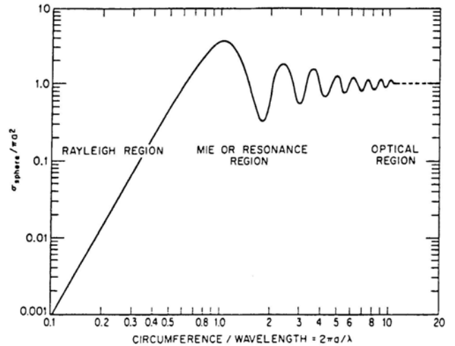
Fig. 1. Sphere RCS versus frequency [7].
