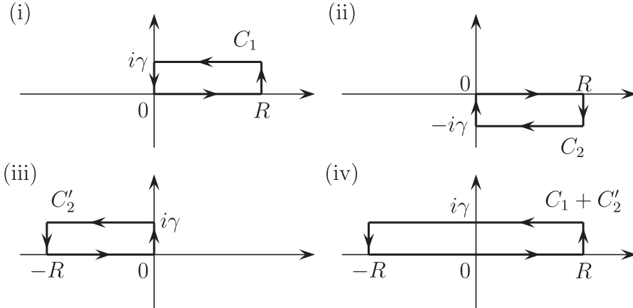
Fig. 2. Integration contours in complex x plane. The endpoint R = \infty for cases (a) and (b), R = \pi for case (c). (For case (c), i\gamma is in the lower half plane because of \gamma = \log q < 0 .)
