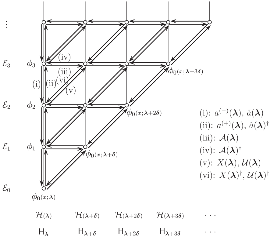
Fig. 1. Shape invariance and Crum's scheme.
