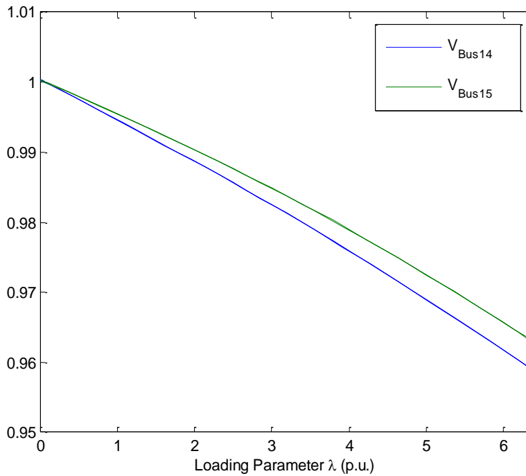
Fig. 9 ( V - \lambda ) Curve obtained bus 14, 15 with connected STATCOM of load bus 14
