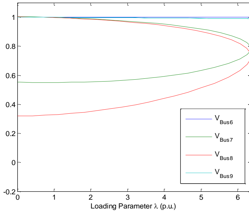
Fig. 11 ( V - \lambda ) Curve obtained bus 6,7,8,9 with connected STATCOM of between buses 6 and 17
