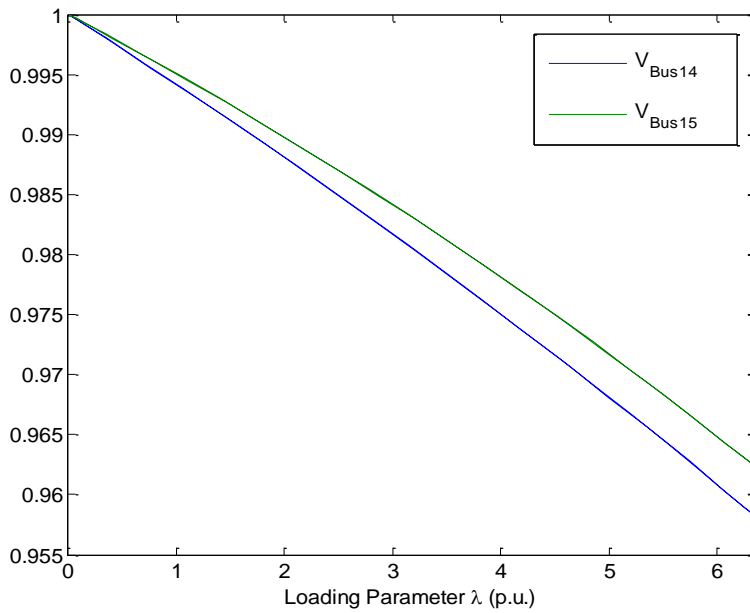
Fig. 12 ( V - \lambda ) Curve obtained bus 14,15 with connected STATCOM of between buses 6 and 17
