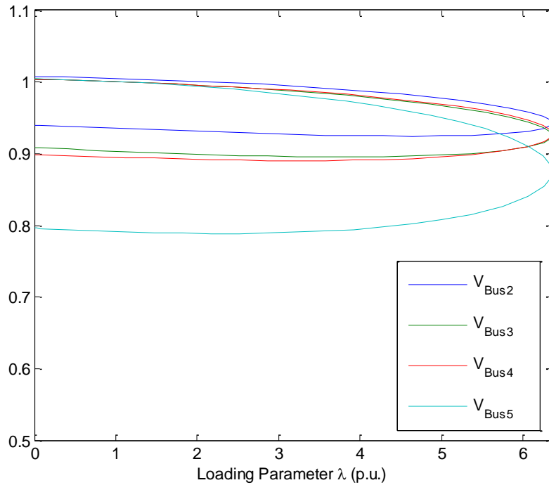
Fig. 10 ( V - \lambda ) Curve obtained bus 2,3,4,5 with connected STATCOM of between buses 6 and 17
