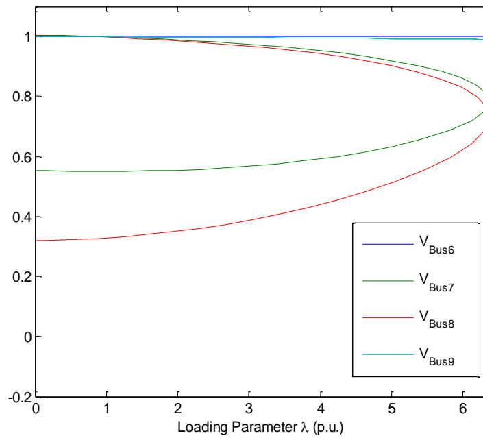
Fig. 7 ( V - \lambda ) Curve obtained bus 6,7,8,9 with connected STATCOM of load bus number 14
