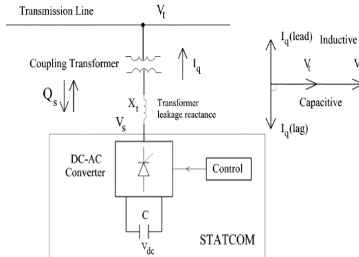
Fig. 1. STATCOM circuit models
