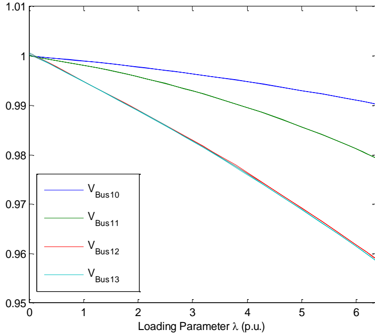
Fig. 8 ( V - \lambda ) Curve obtained bus 10, 11,12,13 with connected STATCOM of load bus 14
