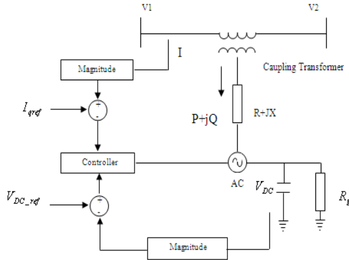
Fig.4. Control model SSSC
