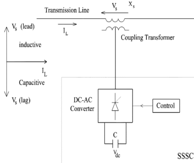
Fig..3 SSSC circuit modeling
