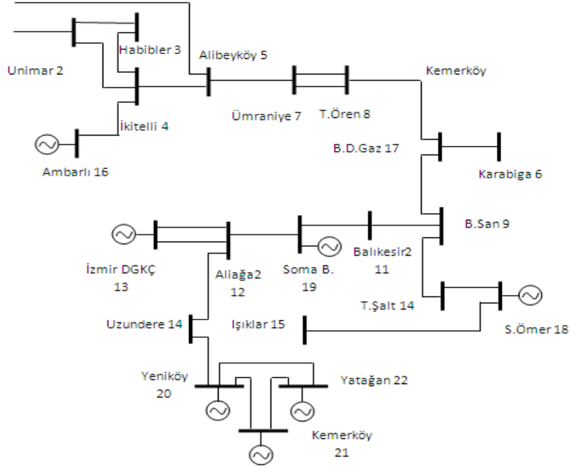
Fig. 5. 22 buses power system models
