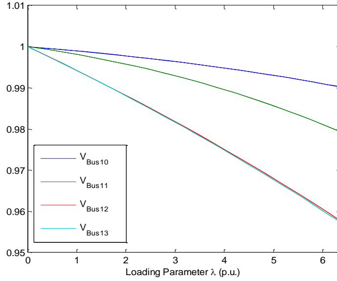
Fig. 12 ( V - \lambda ) Curve obtained bus 10,11,12,13 with connected STATCOM of between buses 6 and 17
