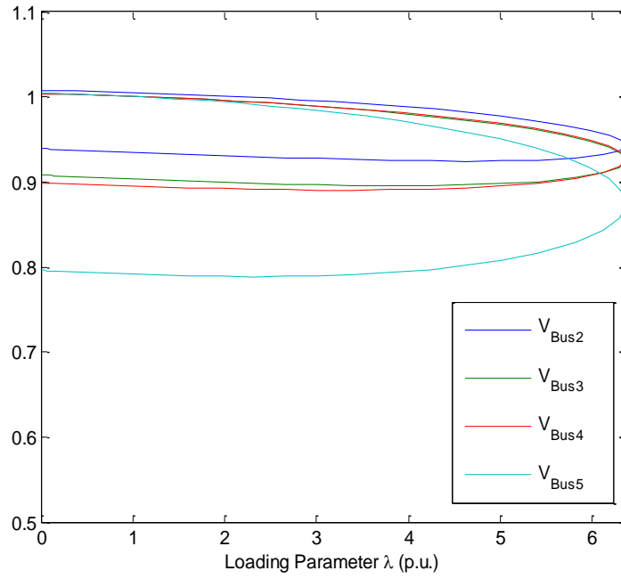
Fig. 6. ( V - \lambda ) Curve obtained bus 2,3,4,5 with connected STATCOM of load bus number 14
