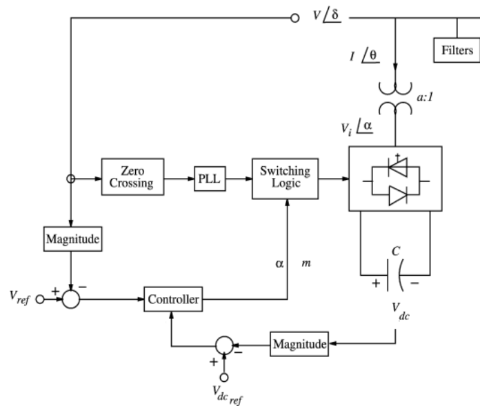
Fig..2 Control model STATCOM
