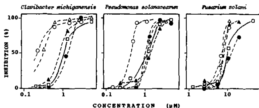
Fig. 4. In vitro inhibition tests with the indicated plant pathogens. The following symbols are used LTP-a1 (●), LTP-a2 (▲), LTP-s1 (○), LTP-s2 (Δ), α1+β thionin from wheat (□).
