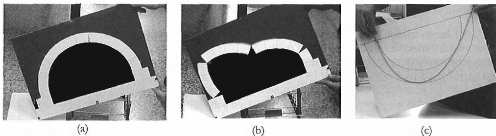
Figure 12 Collapse of an arch under constant horizontal acceleration
