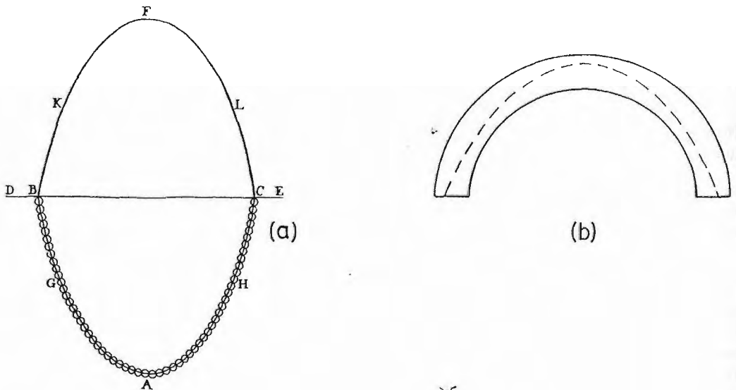
Figure 1 Hooke's analysis of the arch (Heyman 1995)
