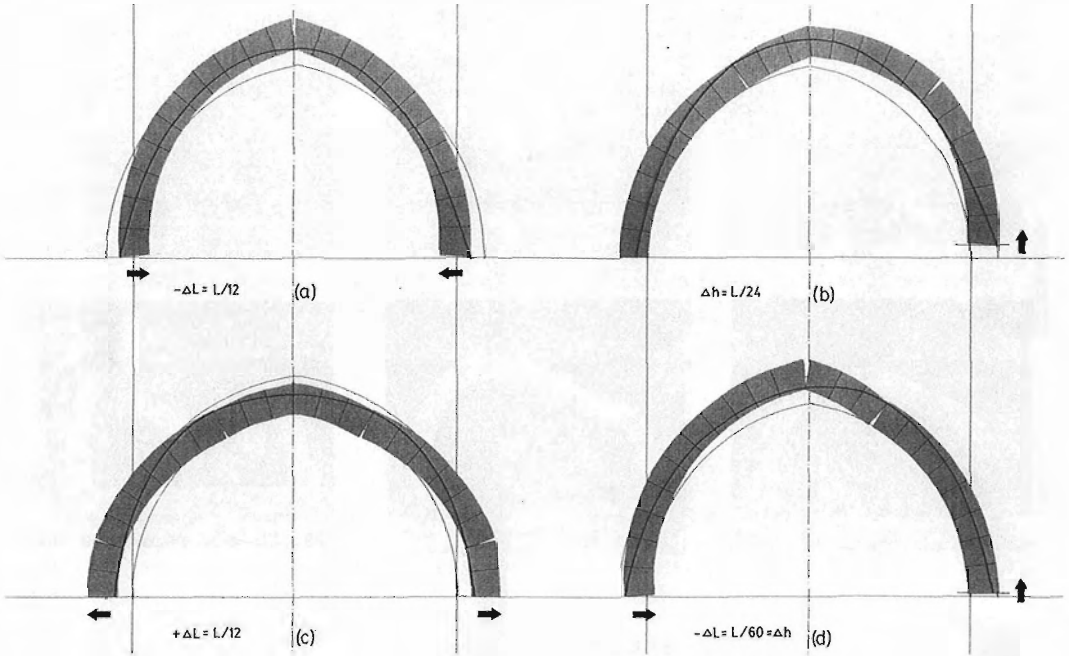
Figure 5. Response of a pointed arch to movements of the supports. Cracking and lines of thrust
