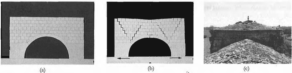
Figure 10 Arch which supports an ashlar wall.
