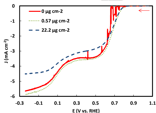
Figure 1. Impact of Nafion ® loading on the electrocatalytic performance of NOMC, measured on a RRDE in an O 2 -saturated 0.1 M KOH solution with a scan rate of 10 \text{ mV s}^{-1} at 2500 rpm. The red arrow indicates the scan direction. J was determined based on the geometric surface area of the disk ( A_{\text{geo}} \approx 0.20 \text{ cm}^2 ).
