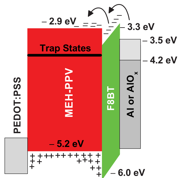
FIG. 2. This sketch shows the energy diagram for fabricated bilayer devices in which the LUMO of F8BT forms an energetic staircase for electron injection from cathodes like Al ( -4.2 eV) or \text{AlO}_x ( \sim -3.5 eV). Ba/Al can form an Ohmic contact with either MEH-PPV or F8BT.
