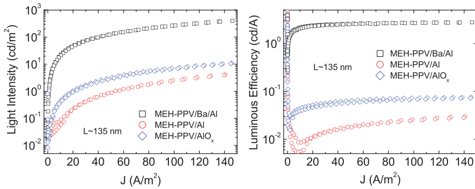
FIG. 1. (a) Light-output versus device current and (b) luminous efficiency of the single-layer and with Ba/Al, Al, and \text{AlO}_x cathodes.
