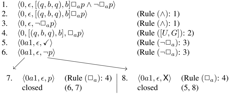
Figure 6.5: Closed tableau for the formula [(q, b, q), b] \Box_a p \wedge \neg \Box_a p
