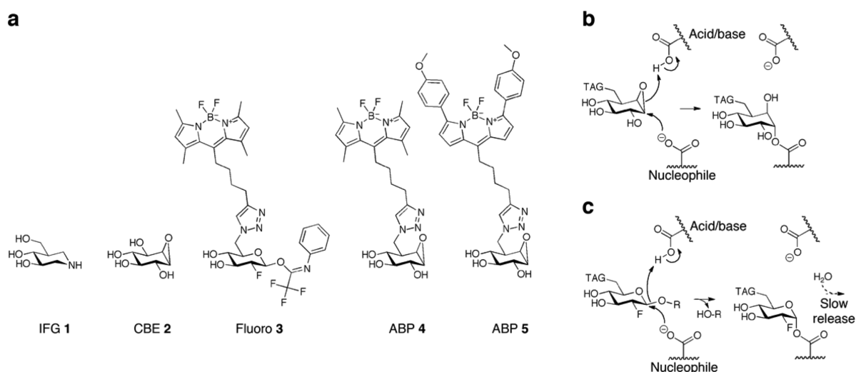
Figure 1. Inhibitors and reaction mechanism. (a) Structural formulas of competitive, reversible inhibitor isofagamine (IFG 1), irreversible inhibitors conduritol β-epoxide (CBE 2), semi-irreversible inhibitor 2-deoxy-2-fluoro-β-D-glucopyranosyl-N-phenyltrifluoroacetimidate 33 (fluoro 3), cyclophellitol β-epoxide type ABP 4 (MDW933, green fluorescent), and β-epoxide-type ABP 5 (MDW941, red fluorescent). 35 (b) Irreversible binding mechanism of β-epoxide-type ABPs to the nucleophile of GBA via its double-displacement mechanism. (c) Hydrolysis of fluoro 3 and temporary trapping of the glycosylated nucleophile adducts of GBA.
