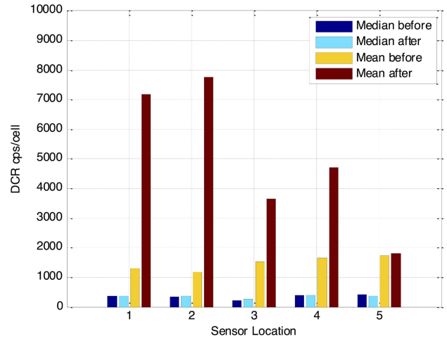
Fig. 3. Mean and median DCR (counts/s per microcell) before and after irradiation of in-room dSiPM-based PET detectors.
