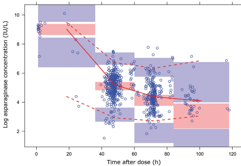
Figure 3. Visual predictive check. Prediction corrected (Pred Corr) visual prediction plot of observed log asparaginase concentrations versus time after last Erwinia asparaginase dose in hours (h) of the final model. Red solid line shows the median observed concentrations and the surrounding opaque red area the simulation based 95% interval for the median. Red dashed lines indicate the observed 5% and 95% percentiles; surrounding opaque blue areas show the simulated 95% confidence intervals for the corresponding predicted percentiles.
