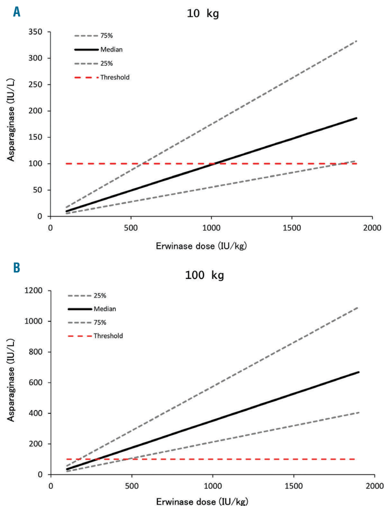
Figure 4. Simulated Erwinia asparaginase concentrations for a 10 kg and a 100 kg patient. Median and the 25% and 75% percentiles of the patients who achieve asparaginase concentrations (y-axis) after 48 hours for different Erwinia asparaginase doses (x-axis). (A) Concentrations for a 10 kg patient and (B) a 100 kg patient. Red dashed line is the target trough concentration of 100 IU/L.
