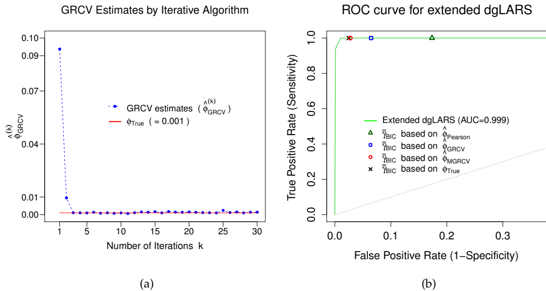
Figure 3.1: (a) GRCV estimates, \hat{\phi}_{GRCV}^{(k)} , produced by the iterative GRCV algorithm based on a simulated data set from Gamma model. (b) ROC curve of the extended dgLARS method computed by averaging over the 50 simulations along with some selected tuning parameters.
