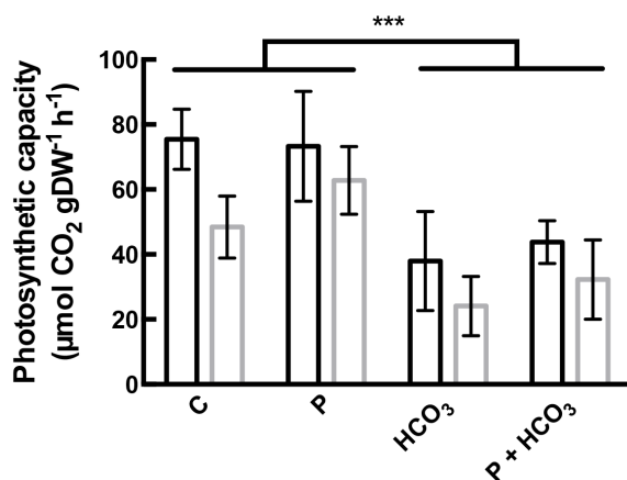
Figure 4. Photosynthetic rates of Sphagnum squarrosum (dark bars) and S. palustre (grey bars) under different surface water treatments. Displayed is the mean \pm SE ( N = 4 ). \text{HCO}_3^- significantly decreased rates, shown by *** P < 0.001 .
