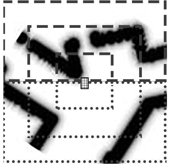
Fig. 2. The window structure of the HoG. The underlying picture is a sample projected cost map. The middle rectangle is the robot footprint and with its rotational axis point in the middle of the image. Each rectangular section is used to calculate the HoG features. This way, the resulting descriptors are more suitable for our problem.
