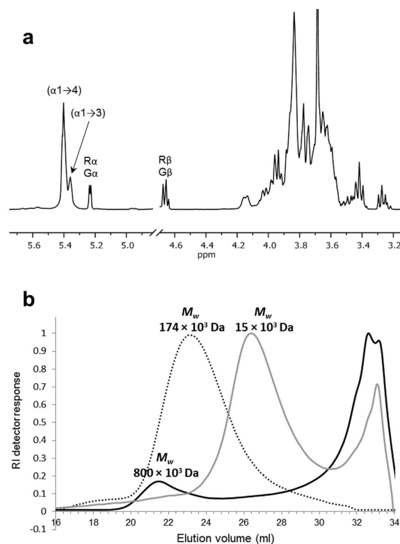
Figure 5. Structural analysis of the products synthesized by the incubation of 0.6% (w v -1 ) amylose V with 25 μg ml -1 of L. fermentum NCC 2970 GtfB for 24 h at 37 °C and pH 5.5. (a) 1 H NMR spectra (D 2 O, 300 K) of the product mixtures formed. The anomeric signals indicated as G α /β and R α /β correspond to free glucose and reducing -(1 → 4)-D-Glcp units, respectively. Chemical shifts are given in parts per million relative to the signal of internal acetone (δ 2.225). (b) HPSEC molecular mass distribution of the reaction products generated from amylose V by the L. fermentum NCC 2970 GtfB enzyme. The elution profiles of the starting amylose V substrate (dashed line) and of the products synthesized by L. reuteri 121 GtfB from amylose V (grey line) are also included.
