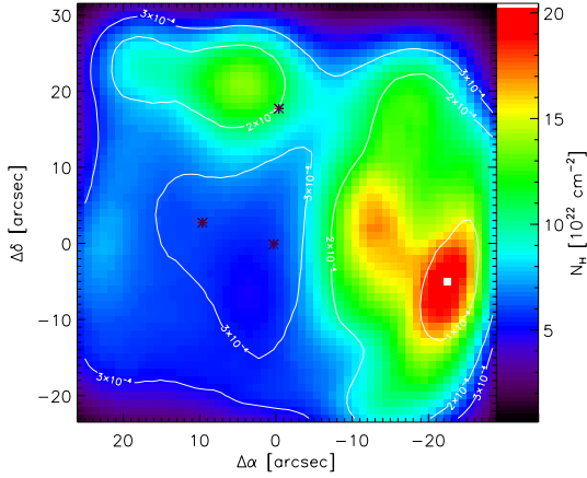
Fig. 10. Column density map of gas derived from FORCAST, PACS, and SCUBA continuum observations in the center of the region (colors), overlaid by contours of the CO abundance, running from 1 \times 10^{-4} to 3 \times 10^{-4} .
