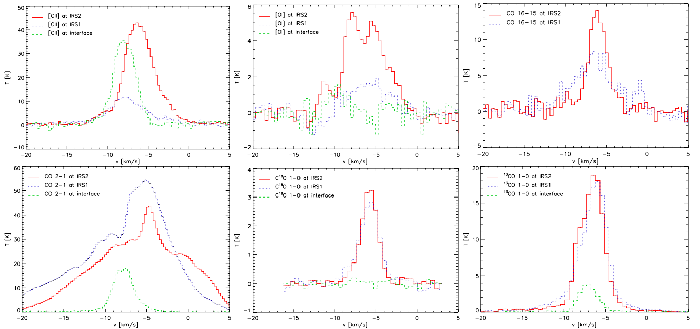
Fig. 6. Line profiles of the [\text{C II}] , [\text{O I}] , \text{CO} 16–15, \text{CO} 2–1, \text{C}^{18}\text{O} 1–0, and ^{13}\text{CO} 1–0 lines at the position of the [\text{O I}] peak (0, 20 close to IRS 2), at IRS 1 (0, 0), and at the interface ( -40 , -54 ). The lines are averaged in a Gaussian beam of 17.3'' FWHM (telescope + convolution kernel) except for the ^{13}\text{CO} and \text{C}^{18}\text{O} lines that can only be treated at the lower resolution of 23'' .
