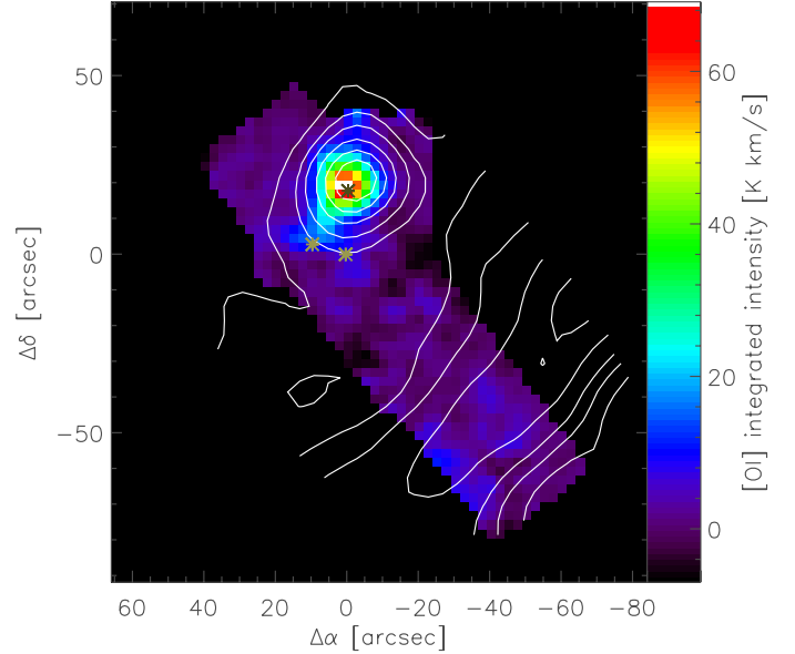
Fig. 3. Integrated intensity map of the [O I] 63 \mu\text{m} line (colors) overlaid by contours of the [C II] integrated intensity (levels as in Fig. 1). The three marks indicate the positions of IRS 1–3. All coordinates are taken relative to the position of IRS 1 at RA = 22 ^{\text{h}} 19 ^{\text{m}} 18 ^{\text{s}} .21, Dec = 63 ^{\circ} 18'46".9 (J2000).
