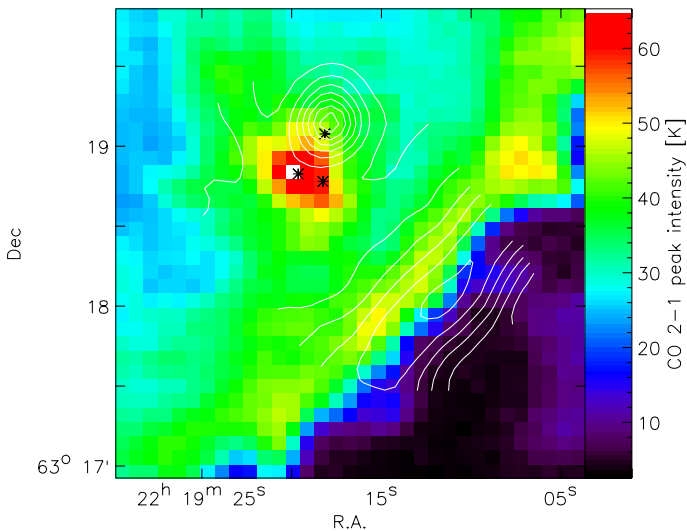
Fig. 2. Peak intensity map of [C II] overlaid on a IRAM 30 m map of the CO 2–1 peak intensity. The [C II] contours are drawn at 15, 20, 25, 30, 35, 40, and 45 K. The black marks indicate the positions of IRS 1–3.
