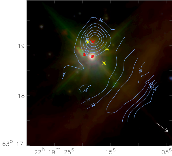
Fig. 1. Integrated intensity map of [C II] overlaid on a Spitzer IRAC false-color image of the same region. The IRAC map uses the logarithmic intensities of the 3.6, 5.6, and 8 \mu\text{m} channels. The integrated intensity contours are drawn at 50, 70, 90, 120, 150, and 180 K km s ^{-1} . The external cloud interface is visible in the southwest. The arrow shows the direction towards the illuminating source HD 211880. The red marks indicate the position of the known infrared sources: southwest is IRS 1, north is IRS 2, and southeast is IRS 3 (Evans et al. 1989), the yellow marks show the position of known submm cores (Minchin et al. 1995; Maud et al. 2013). The IRAC peak falls at the location of IRS 1.
