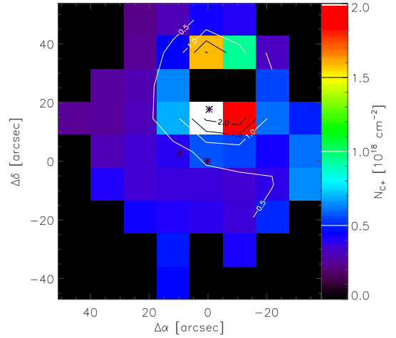
Fig. 11. Column density map of \text{C}^+ derived from the measured [C II] intensities using the gas parameters from the RADEX fit to the CO lines. The contours show the [C II] line optical depth at levels of \tau = 0.5, 1.0, 1.5, 2.0 . In the two pixels north of IRS 2, the optical depth is too large for a reliable column density estimate.
