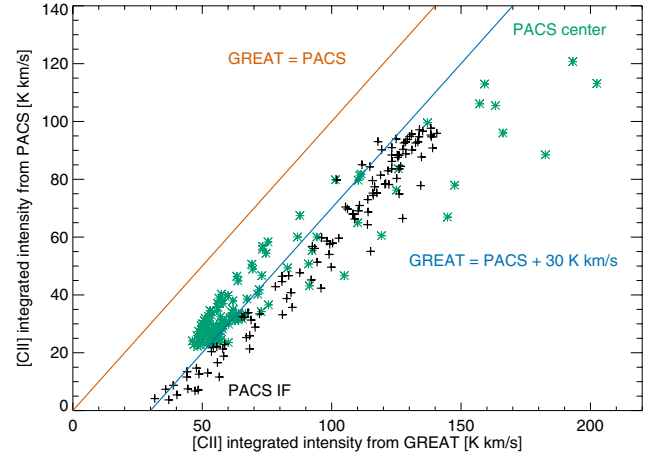
Fig. A.2. Measured intensities in the different pixels from Fig. A.1b as seen by GREAT and PACS. Green asterisks represent the footprint around IRS 1, black plus signs the footprint at the outer interface. The brown line shows the identity, the blue line represents an identity with an offset of 30 K km s -1 .
