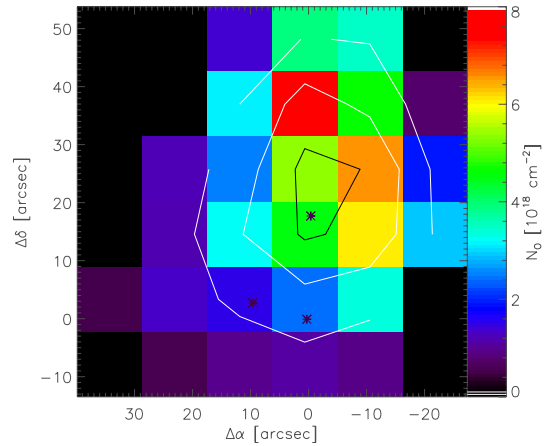
Fig. 12. Column density map of atomic oxygen derived from the measured [O I] intensities using the gas parameters from the RADEX fit to the CO lines. The contours show the [O I] line optical depth at levels of \tau = 0.05, 0.10, 0.15, 0.20 .
