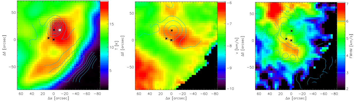
Fig. 5. Peak intensity, first moment (centroid velocity), and second moment (translated to FWHM) of the lines of ^{13}\text{CO} 1–0 (colors) and [\text{C II}] contours. The black marks indicate the positions of IRS 1–3. The contour levels for the [\text{C II}] peak intensity match those from Fig. 2; for the line position they are given at -9.5 , -8.5 , -7.5 , and -6.5 \text{km s}^{-1} , and for the line width at 3, 4, 5, and 6 \text{km s}^{-1} . Velocities are given in LSR (local standard of rest) and intensities in main beam temperatures.
