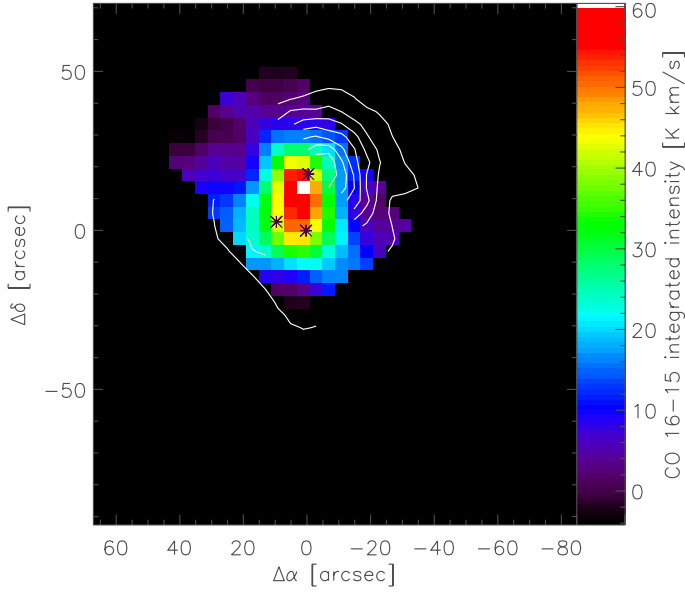
Fig. 4. Integrated intensity map of CO 16–15 with contours of CO 13–12 drawn at levels of 10, 20, 30, 40, 50, 60, and 70 K km s -1 . Only the region around IRS 1 has been observed in CO 16–15; in CO 13–12 only two outer strips have been covered avoiding the center. The black marks indicate the positions of IRS 1-3.
