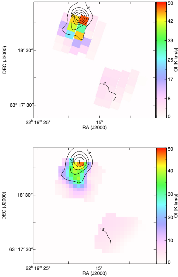
Fig. A.3. Integrated map of [O I] obtained in the GREAT observations (contours) overlaid on the colors of the [O I] line intensity from the two PACS footprints. The top image shows the intensities in the original PACS footprints with GREAT data convolved to 10'' resolution. In the bottom version both maps are resampled to the positions of the GREAT map for the effective resolution of a circular 12'' beam.
