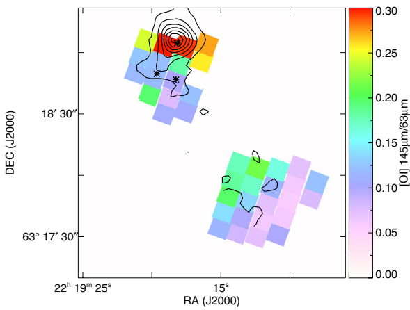
Fig. B.1. Observed ratio of the [O I] 145 \mu\text{m} to [O I] 63 \mu\text{m} line integrated intensity seen by PACS (colors) overlaid on the contours of the [O I] 63 \mu\text{m} emission measured by GREAT.
