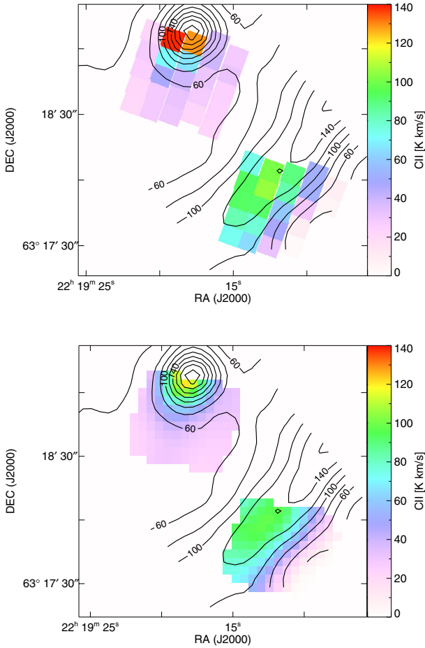
Fig. A.1. Integrated map of [C II] obtained in the GREAT observations (contours) overlaid by colors of the [C II] line intensity from the two PACS footprints. The top image shows the intensities in the original PACS footprints. In the bottom version this is resampled to the positions of the GREAT map with an effective resolution of the 17.2'' beam.
