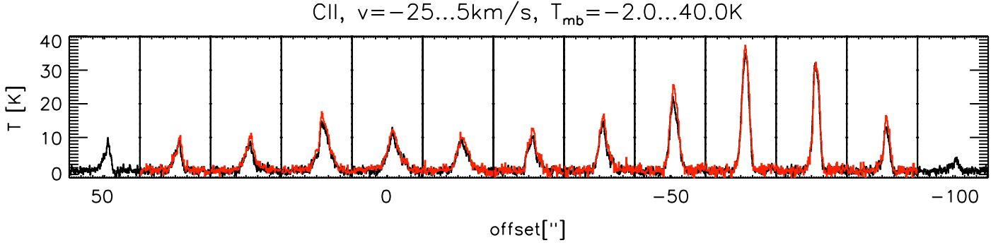
Fig. A.5. [C II] spectra taken with HIFI (black) and GREAT (red) along a 37 degree cut through IRS 1 and the cloud surface. The HIFI cut extends deeper into the cloud and only every second spectrum is plotted. The corresponding GREAT spectra were averaged in a 6'' circle around the HIFI position.
