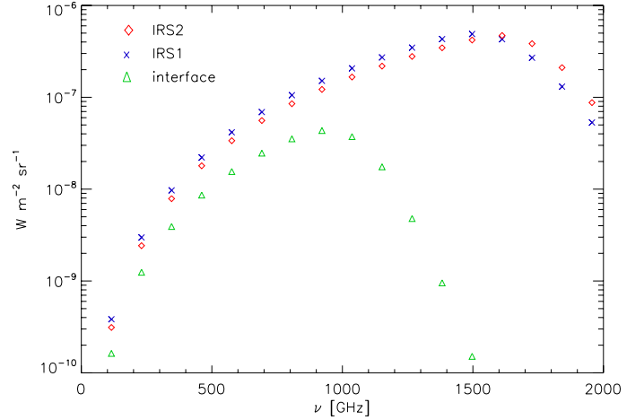
Fig. 14. CO ladder from the RADEX fit to the line intensities at the three prominent positions.
