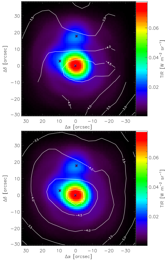
Fig. 15. Comparison of the line cooling with the infrared continuum cooling. The background colors show the total infrared flux integrated from wavelengths starting at 11 \mu\text{m} (Koumpia et al. 2015). The contours give the decadic logarithm of the ratio of the integrated line flux relative to the continuum flux. In the top panel we use the sum of the [O I] and [C II] fluxes, in the lower panel , we only show the [C II]/TIR ratio as used in many existing investigations.
