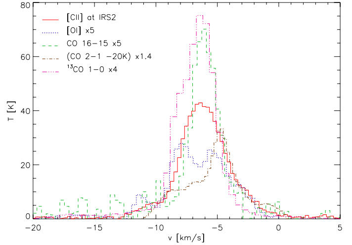
Fig. 8. Line profiles of the [C II], [O I], CO 2-1, CO 16-15, and ^{13}\text{CO} 1-0 lines at the position of the [O I] peak (0, 20). The lines were scaled to similar intensities at -4 \text{ km s}^{-1} . For CO 2-1, a constant emission of 20 K is subtracted to exclude the extended outflow emission.
