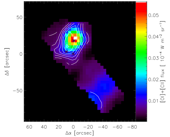
Fig. 16. Comparison of the total line cooling flux provided by the sum of the [O I] and [C II] lines (colors) to the [O I]/[C II] line flux ratio (contours from 0.4 to 2.8 in steps of 0.4). The computation is performed in a common effective beam of 15'' .
