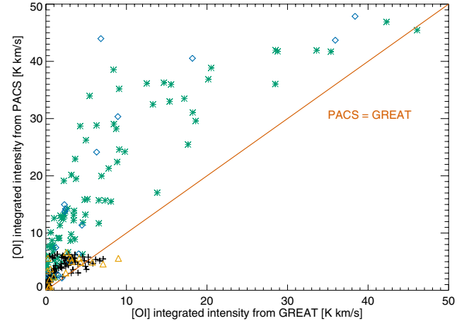
Fig. A.4. Measured intensities in the different pixels of Fig. A.3 as seen by GREAT and PACS. Green asterisks represent the footprint around IRS 1 and black plus signs the footprint at the outer interface when both data sets are resampled to a common 12'' resolution (Fig. A.3b). Blue diamonds and orange triangles are obtained when we resample the GREAT data to the 25 pixels of the PACS array using the 9'' PSF of PACS for the IRS 1 region and the interface, respectively (Fig. A.3a). The brown line shows the identity.
