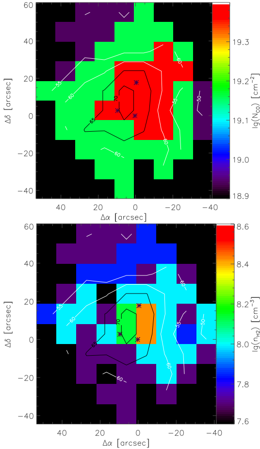
Fig. 9. CO column density ( upper plot : colors), gas density ( lower plot : colors), and kinetic temperature (both plots: contours) derived from the RADEX fit of the integrated intensities of the observed lines of CO 1–0, 2–1, and 16–15 and the isotopologues ^{13}\text{CO} 1–0 and \text{C}^{18}\text{O} 1–0.
