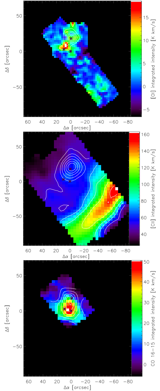
Fig. 13. Intensity map of [O I] (top), [C II] (center), and CO 16–15 (bottom) after subtracting a Gaussian intensity distribution of FWHM = 8.3'' from the observed map. The overlaid contours show the original intensity maps at levels of 8, 24, 40, 56, and 72 \text{K km s}^{-1} ([O I]); 50, 70, 90, 120, 150, and 180 \text{K km s}^{-1} (CII); and 10, 20, 30, 40, 50, and 60 K (CO 16–15).
