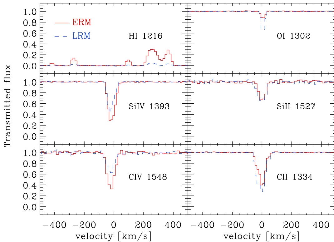
Figure 17. Synthetic spectra extracted from the l.o.s. drawn through the simulated box with physical properties shown in Fig. 16. The spectra are calculated using an early reionization model (ERM, red solid line) and a late reionization model (LRM, blue dashed line) for Ly \alpha forest (upper-left panel) and metal absorption lines (O I, upper-right panel; Si IV and Si II, middle-left and middle-right panel; C IV and C II, lower-left and lower-right panel, respectively). See the text for the definitions.
