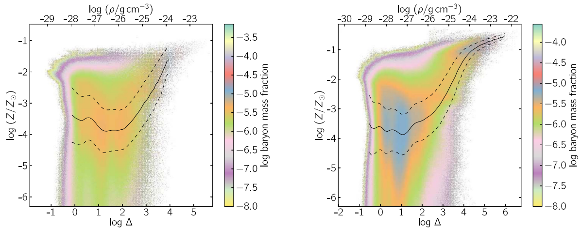
Figure 11. Mass-weighted probability distribution function (PDF) of the baryons at z = 6 (left) and z = 4 (right) in the metallicity–overdensity plane. The solid (dashed) black line is the mean (rms) metallicity as a function of density.
