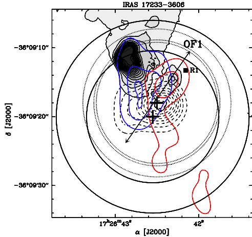
Fig. 1. Grey scale and solid black contours represent the H 2 emission at 2.12 \mu\text{m} ; dashed contours are the 1.4 mm continuum emission. Red and blue contours are the SMA integrated emission of the SiO(5–4) line ( v_{\text{bl}} = [-30, -20] km s -1 and v_{\text{rd}} = [+10, +39] km s -1 ). The crosses mark the Herschel pointings; the solid and dotted circles are the Herschel beams (Sect. 2). The square marks the peak of the EHV CO(2–1) red-shifted emission (R1). The arrow marks the OF1 outflow.
