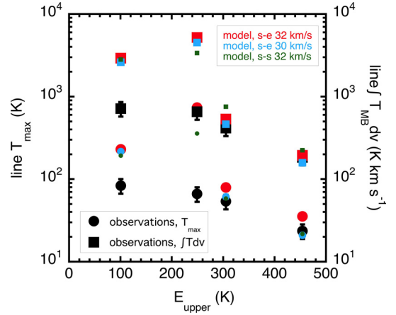
Fig. B.1. Observed and modelled maximum brightness temperatures (circles), and integrated intensities (squares) for the blue-shifted emission. Data points (in black) are corrected for an emission region of 3 \text{ arcsec}^2 and for 60% of the emission due to OF1. Errorbars are \pm 20\% of the observed value. Three models are shown: the model of Paper II with level populations in statistical equilibrium (“s-e” in red) with v_s = 32 \text{ km s}^{-1} , one with a slower shock velocity ( v_s = 30 \text{ km s}^{-1} , blue), and a model in stationary-state (“s-s” in green).
