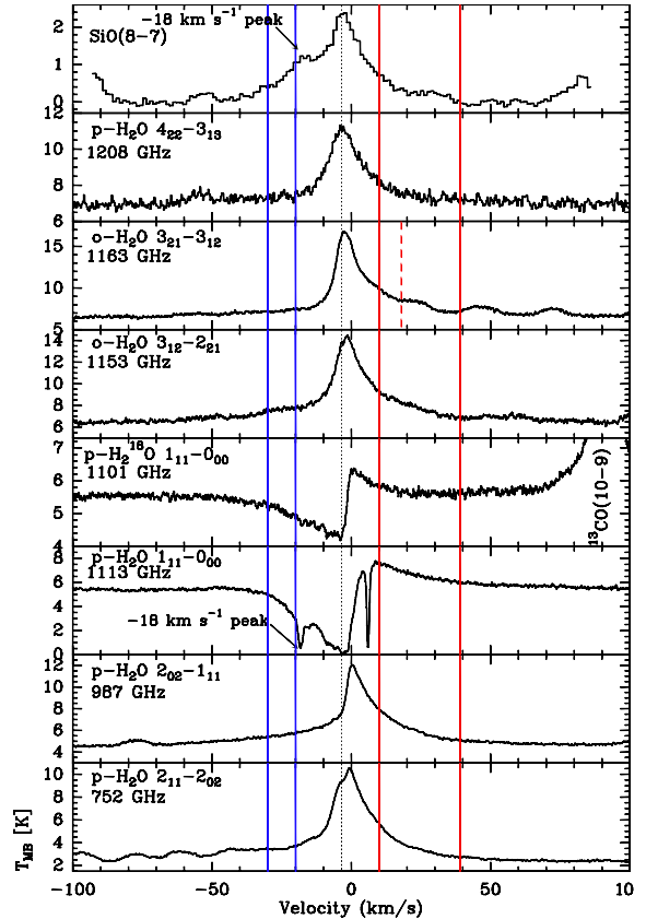
Fig. 2. Spectra of the water lines and of the SiO(8–7) transition towards IRAS 17233–3606. In all Herschel spectra, the continuum level is divided by a factor of two to correct for the fact that HIFI operates in double-sideband. The red and blue lines mark the velocity range used for the modelling of the water emission (solid red: [+10, +39] km s -1 ; dashed red: [+18] km s -1 ; blue: [-30, -20] km s -1 , Sect. 4). The SiO(8–7) spectrum has a beam size of 18'', similar to the 19'' beam size of the 1113 GHz line, and it is observed at (4'.7, 0'.0) from the Herschel \alpha_{\text{J2000}} = 17^{\text{h}}26^{\text{m}}42^{\text{s}}:54 , \delta_{\text{J2000}} = -36^{\circ}09'20''.00 pointing. The dotted line marks the ambient velocity.
