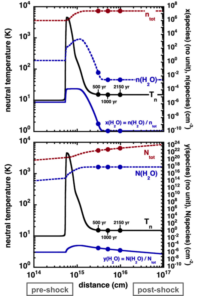
Fig. A.1. Upper panel: neutral temperature (black curve), total density (red dashed curve), water density (blue dashed curve), and fractional density (blue continuous curve). The so-called fractional density is the water density over the total density, locally defined at each point of the shock. Lower panel: neutral temperature (black curve), total column density (red dashed curve), water column density (blue dashed curve), and fractional column density (blue continuous curve). The so-called fractional column density is the water column density over the total column density. The column density (in \text{cm}^{-2} ) is the integral of the local density (in \text{cm}^{-3} ) along the shock width (in cm). In both panels, the three points labelled on each curve correspond to the distance parameter of 3.1 \times 10^{15} , 5.15 \times 10^{15} , 10^{16} cm, or to time parameters values of 500, 1000, and 2150 yr.
