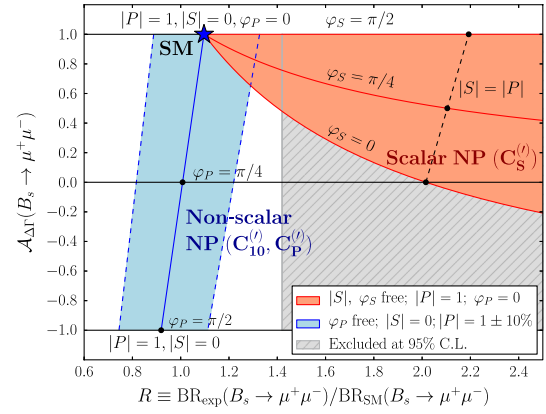
FIG. 2 (color online). Illustration of allowed regions in the R - \mathcal{A}_{\Delta\Gamma} plane for scenarios with scalar or nonscalar NP contributions.
