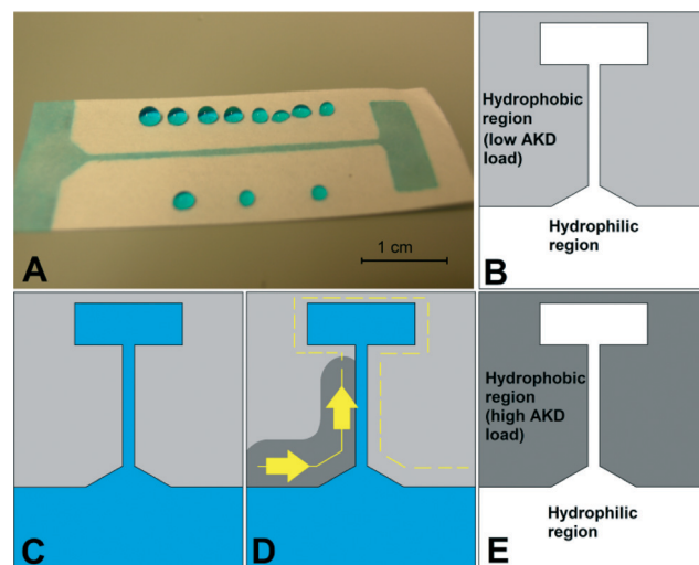
Fig. 2 Second application of AKD (5.0 g L -1 ) to increase hydrophobicity. (A) Paper device after the first low-load AKD application step. An aqueous blue dye solution was applied to both the hydrophilic and hydrophobic domains to demonstrate wettability by water. The hydrophilic domains were wetted, whereas the solution formed droplets on top of the hydrophobic areas. (B) Schematic design of the device in A. (C) The hydrophilic area was wetted with water for the second AKD application. (D) A 5.0 g L -1 hexane solution of AKD (high-load) was applied via a syringe on a pump to the hydrophobic domain, by manually moving a flexible capillary tip along the borders between the hydrophilic and hydrophobic regions. As the hydrophilic regions were filled with water, the hexane containing AKD did not enter into those regions (hydrophilic exclusion). Afterwards, the paper was put into the oven at 80 °C for 3 min. (E) The hydrophobic regions became more hydrophobic, whereas the hydrophilic regions remained unchanged.
