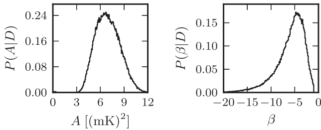
Figure 10. Marginalized probability densities for the scaling amplitude A and the power-law index \beta . A rises to a significance of four standard deviations above the null hypothesis in 600 h of integration.
