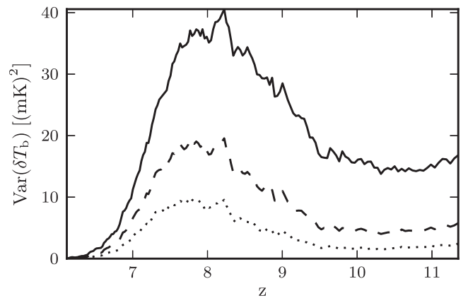
Figure 1. Evolution of the variance of the EoR signal, i.e. the 21-cm differential brightness temperature ( \delta T_b ) with redshift, as predicted by a simulation with 21CMFAST. From top to bottom, the curves correspond to decreasing spatial resolutions of 3 (resolution of the LOFAR core, i.e. the central 2 km of the array at 150 MHz, z \approx 8.5 ), 7 and 12 arcmin. The resolution is expressed as the FWHM of the Gaussian kernel that was used to smooth the simulation maps.
