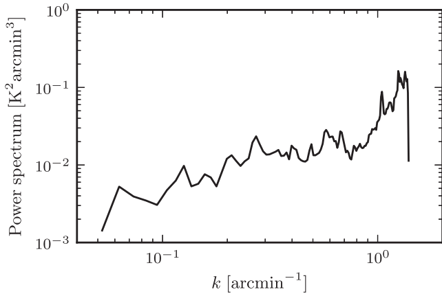
Figure 5. Radially averaged two-dimensional power spectrum of the noise at 150 MHz as a function of wavenumber k = 2\pi/\theta , where \theta is the angular scale. Most of the noise power is concentrated at large k values due to the lower sampling density of the outer part of uv plane.
