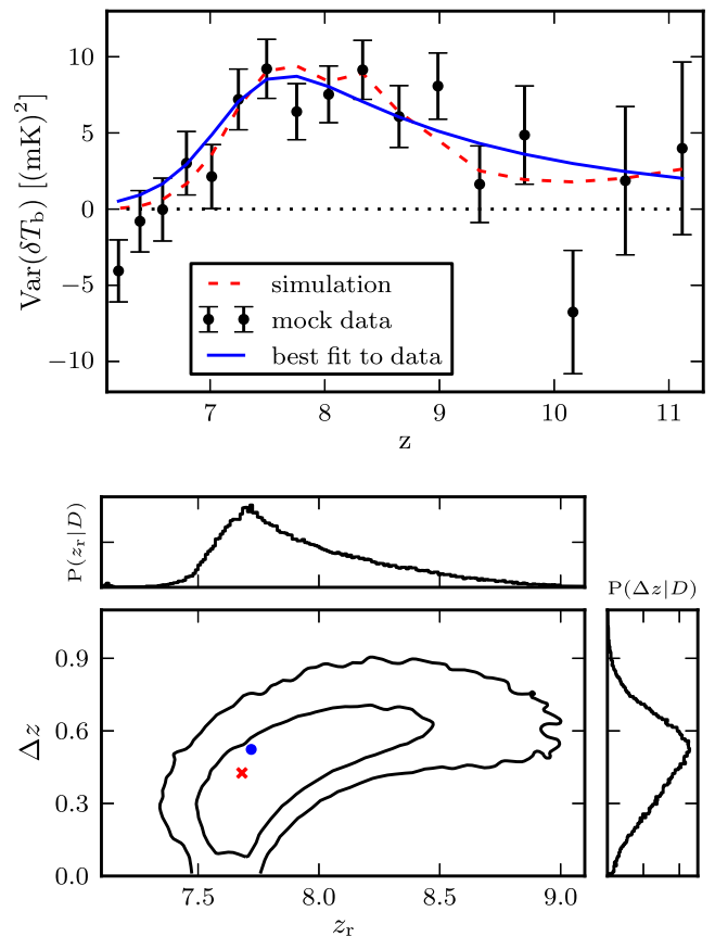
Figure 9. Model fitting and parameter estimation results for a mock data set of 600 h of integration. Top panel: variance of \delta T_b as a function of redshift. Dashed curve: original EoR signal; black points: estimated variance; solid curve: model fit to the data. Error bars are calculated from equation (13). Bottom panel: constraints on the reionization parameters with 68 and 95 percent confidence levels. The cross and dot show the actual and best-fitting values of the parameters, respectively. Marginalized probability densities are plotted on the sides.
