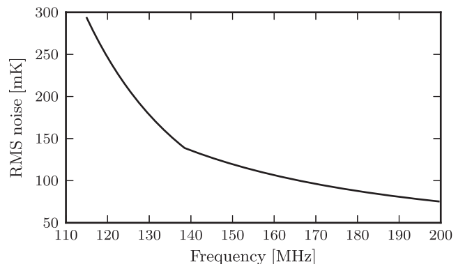
Figure 4. rms system noise as a function of frequency after 600 h and 0.5 MHz integration, used for normalizing the noise simulations.
