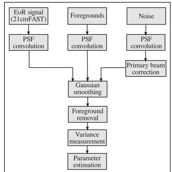
Figure 3. Block diagram of the end-to-end simulation and analysis pipeline.
