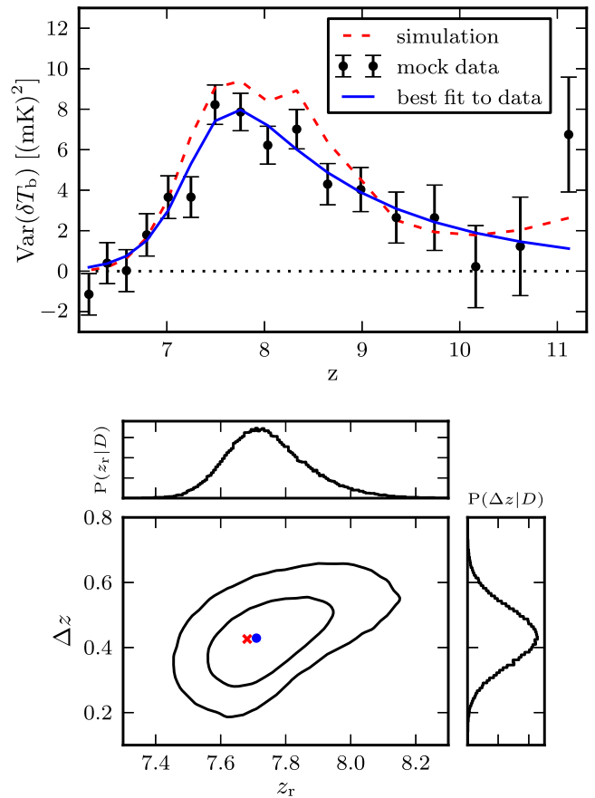
Figure 14. Variance extraction and parameter estimation results for 1200 h of integration. The constraints on reionization parameters improve with better SNR, but the systematic error due to the part of the signal that is removed by foreground removal starts to become significant in the model fitting.
