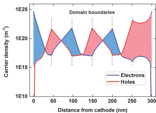
Fig. 5 Carrier concentration profile at short-circuit conditions ( V_{\text{applied}} = 0 V) along the thickness of the vertical device structure as shown in Fig. 3b. The red and blue colored regions show the segregation of holes and electrons respectively, at the domain boundaries.
