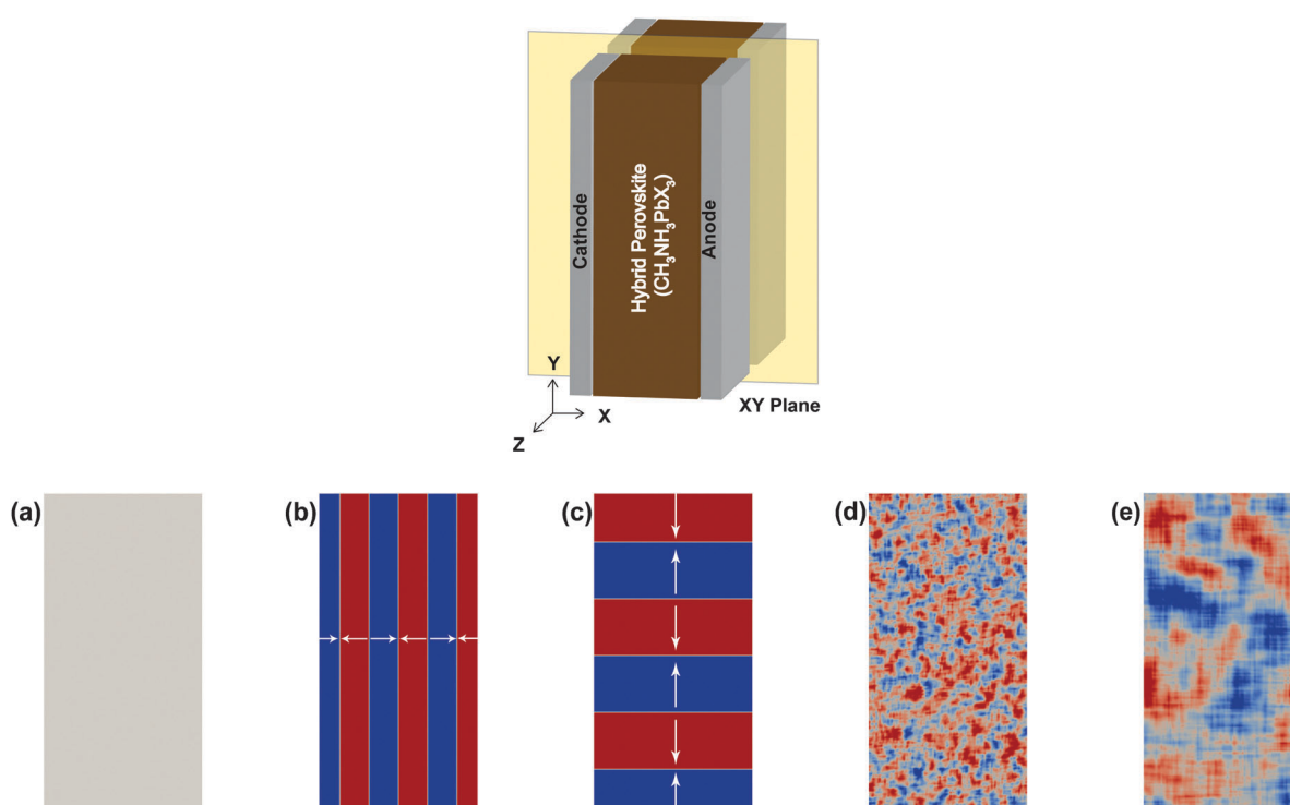
Fig. 3 Cross section of the perovskite solar cell in the X - Y plane showing model ferroelectric domains in the perovskite. The arrows indicate the direction of polarization vector in the respective domains. Assuming high recombination strength, simulations are performed for devices with (a) no polarization, (b) polarization in \pm X direction forming vertical domains, (c) polarization in \pm Y direction forming lateral domains, (d) short order correlated polarization, and (e) long order correlated polarization. The dimensions of all model structures are 300 \text{ nm} \times 600 \text{ nm} \times 600 \text{ nm} . A number of ten realizations are made for the short and long order correlated microstructures.
