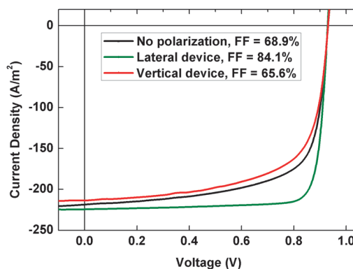
Fig. 4 Simulated J - V curves for device with no polarization (Fig. 3a), vertical device (Fig. 3b) and lateral device (Fig. 3c).
