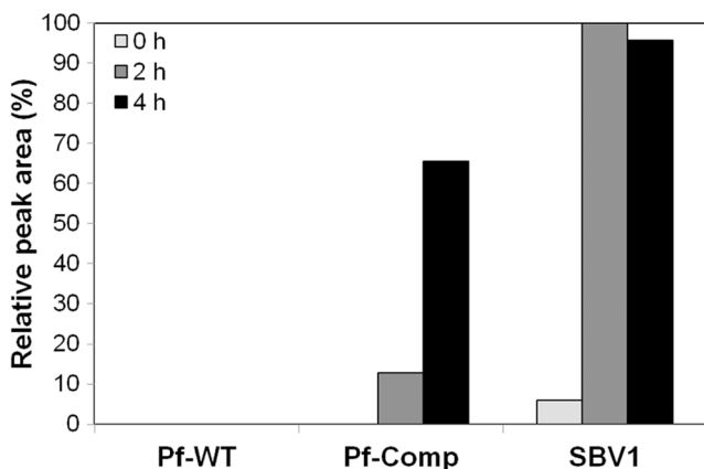
Fig. 3 Conversion of \beta -valine to \beta -valinyl-CoA by cell-free extracts of cells grown on medium supplemented with \beta -valine and ammonium sulfate as nitrogen sources. Relative \beta -valinyl-CoA levels in the samples were analyzed after 0, 2, and 4 h of incubation using HPLC, where \beta -valinyl-CoA levels in SBV1 cell extracts after 2 h incubation was set at 100 %. Pf-WT \beta -valine growth-deficient strain Pseudomonas fluorescens Pf0-1, Pf-Comp P. fluorescens Pf0-1 containing the bvaA gene on the complementing plasmid p4-D1, SBV1 \beta -valine-degrading organism described in this study
