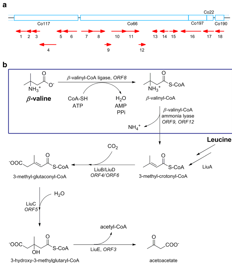
Fig. 1 a Schematic representation of the organization of the ORFs identified in the 26,347 bp insert of plasmid p4-D1. b Proposed degradation pathway of \beta -valine by Pseudomonas sp. SBV1. The boxed region represents the putative initial steps in the \beta -valine degradation pathway, resulting in formation of 3-methyl-crotonyl-CoA, a common intermediate in the leucine degradation pathway, represented in the lower part. ORFs that are putatively important for \beta -valine degradation based on homology to enzymes with known function (Table 1) are numbered
