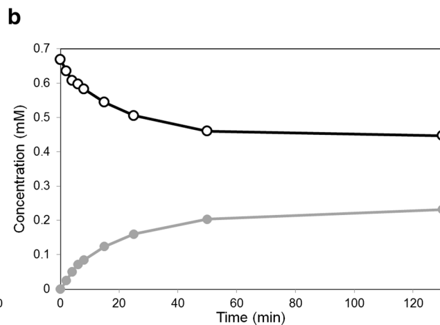
formation of methyl-crotonyl-CoA (closed grey symbols) by purified BvaB1-his in time as monitored by HPLC
