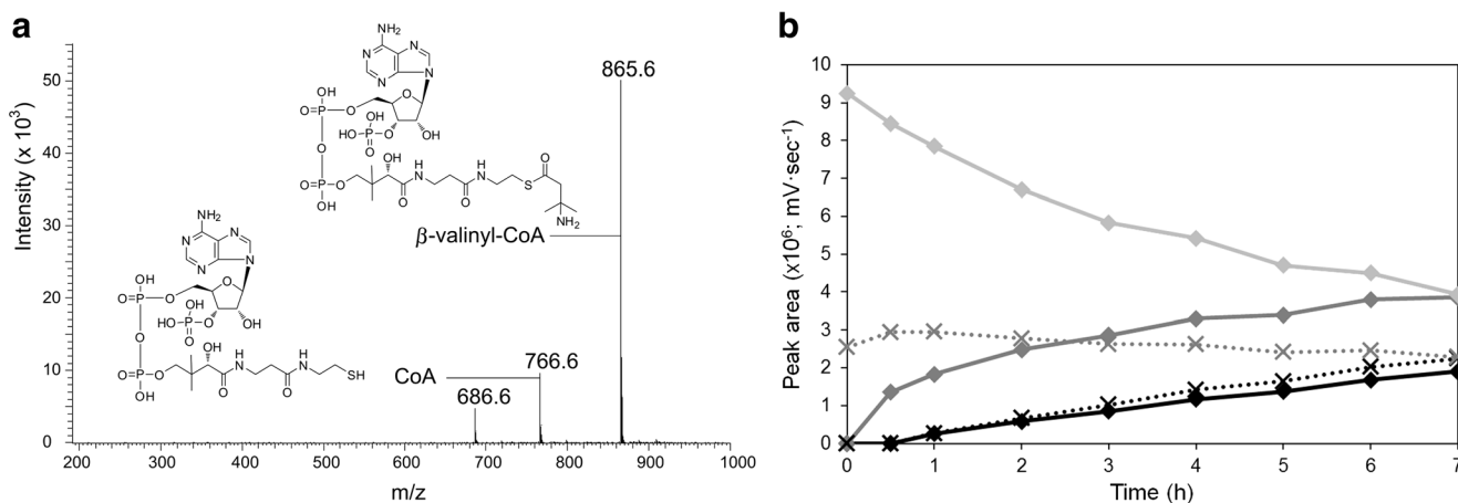
Fig. 2 a MS spectrum of the single protonated form of \beta -valinyl-CoA ( m/z of 866) and CoA ( m/z of 767). b HPLC analyses monitoring the formation of AMP and \beta -valinyl-CoA by BvaA-His in time. Lines: \blacklozenge , AMP; \blacklozenge , ADP; \blacklozenge , ATP. Dotted lines: \times , \beta -valinyl-CoA; \times , CoA
