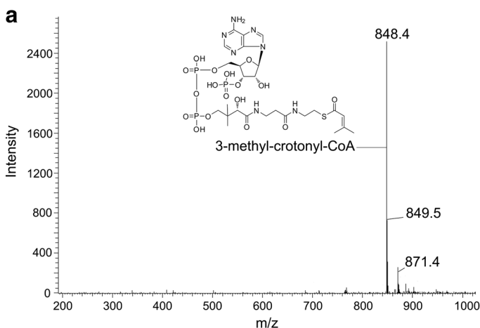
Fig. 4 Identification of \beta -valinyl-CoA ammonia lyase product. a MS spectrum of the single protonated form of 3-methyl-crotonyl-CoA ( m/z 849). b Conversion of \beta -valinyl-CoA (open black symbols) and
