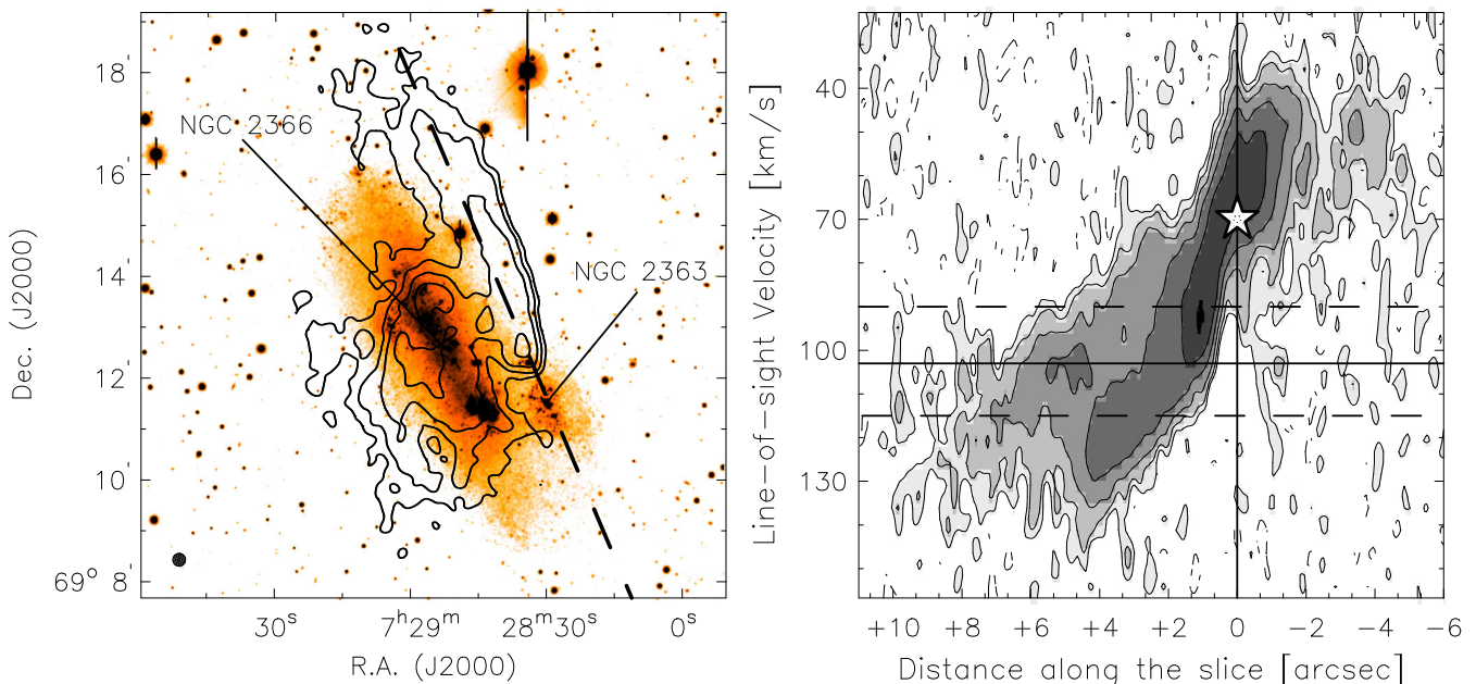
Figure 7. Kinematically anomalous gas in NGC 2363/NGC 2366. Left: V -band image overlaid with the H I emission at 15 arcsec resolution, integrated over a narrow velocity range near the systemic velocity of NGC 2366 (from \sim 90 – \sim 115 km s ^{-1} ). The H I column densities are 2, 4, 8, 16 M_{\odot} pc ^{-2} . The arrows indicate the centres of NGC 2363 and NGC 2366. The circle to the bottom-left shows the H I beam. Right: PV diagram taken along the dashed line shown in the left-hand panel. The solid, horizontal line indicates the systemic velocity of NGC 2366 (103 km s ^{-1} ), while the dashed, horizontal lines show the velocity range that has been used to create the H I map in the left-hand panel. The vertical line corresponds to the spatial position of NGC 2363, while the star shows its optical systemic velocity (70 km s ^{-1} ), as given by NED. Contours are at -1.5\sigma (dashed), 1.5\sigma , 3\sigma , 6\sigma , and 12\sigma , where \sigma = 0.66 mJy beam ^{-1} .
