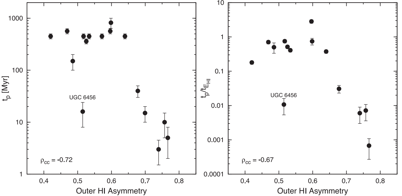
Figure 6. The asymmetry parameter A versus the lookback time t_p at the peak of the SFH (left) and the ratio t_p/t_{E_{HI}} (right), which roughly estimates the number of orbits that the outermost gas has completed since the onset of the starburst. In both panels, the value of the Pearson’s correlation coefficient is indicated. See Section 4.3 for details.
