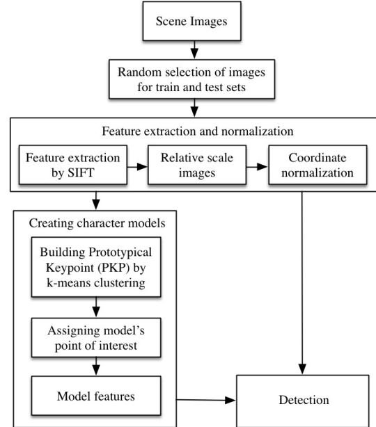
Figure 4: Character modeling architecture
