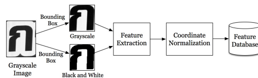
Figure 6: Process flow of feature extraction and coordinate normalization
