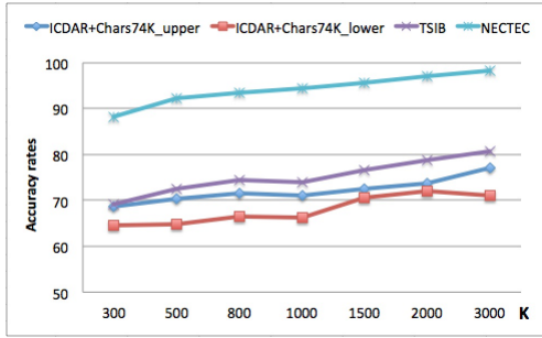
Figure 9: Character recognition results for different values of code book size k (i.e., number of PKPs).
