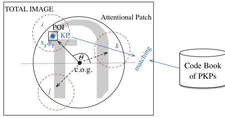
Figure 3: Schematic description of the attentional-patch modeling approach. Center of gravity (c.o.g) \triangleq (0,0)
