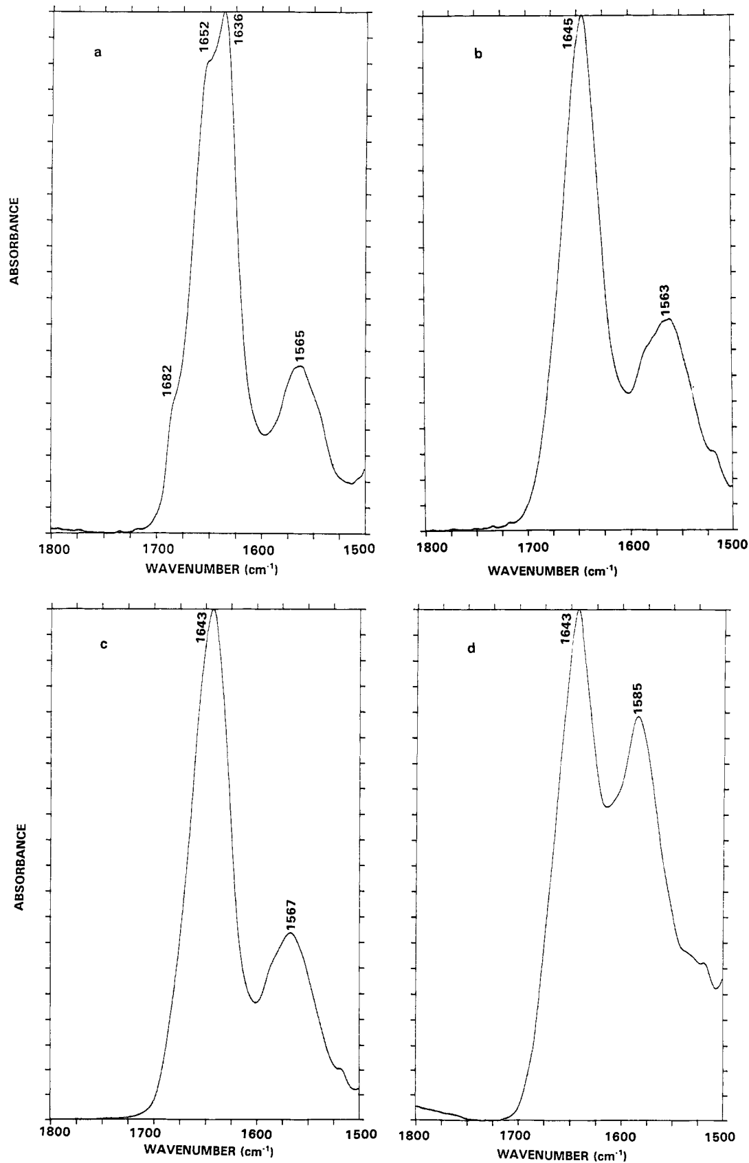
FIGURE 3: Comparison of the FTIR spectra of the HPr and the IIA ml protein when recorded alone and in an interaction involving the two proteins in a 1:1 molar ratio. The spectra were recorded for samples in 2 H 2 O at 20 °C. (a) The absorbance spectrum of the unlabeled HPr protein. (b) The absorbance spectrum of the unlabeled IIA ml protein. (c) The absorbance spectrum of the HPr and the IIA ml protein mixed in a 1:1 M ratio. Both proteins are unlabeled. (d) The absorbance spectrum of the 13 C/ 15 N-labeled HPr protein mixed with unlabeled IIA ml protein. (Note the separation of the two amide I maxima.)
