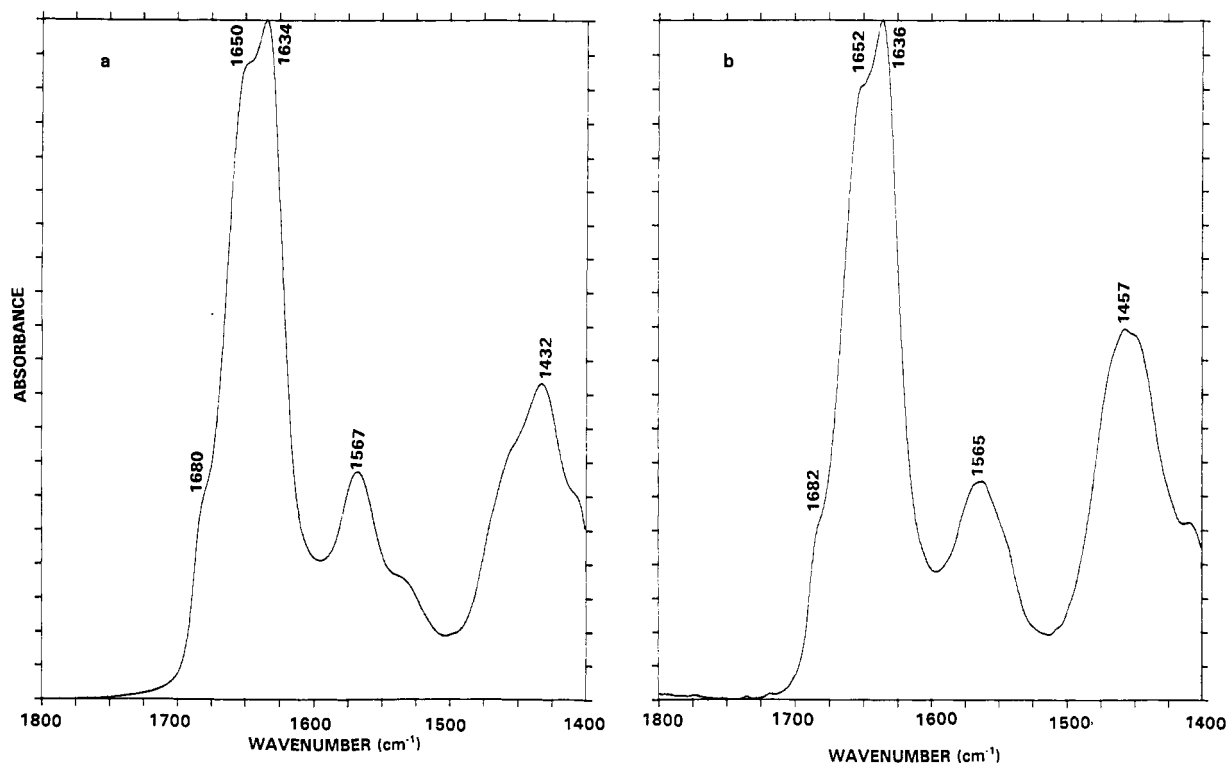
FIGURE 2: Comparison of the FTIR absorbance spectra of ^{15}\text{N} -labeled (a) and unlabeled HPr protein (b) recorded in ^2\text{H}_2\text{O} at 20^\circ\text{C} .
