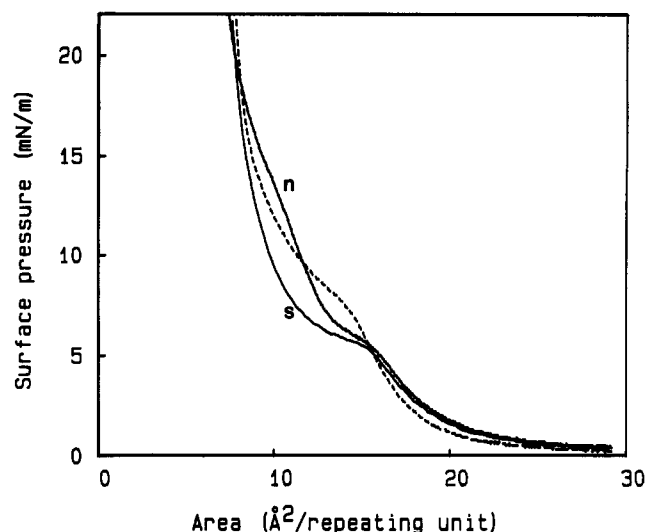
Figure 9. Pressure–area isotherms of a 2:1 mixture of s-PMMA m41 ( M_n 11 000) and i-PMMA m8 ( M_n 36 000), before (n) and after (s) addition of 26 wt % stereoblock PMMA. The dashed line represents pure stereoblock PMMA. T = 45^\circ\text{C} .
