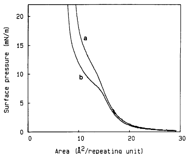
Figure 4. Pressure–area isotherms of stereoblock PMMA: (a) T = 22^\circ\text{C} ; (b) T = 45^\circ\text{C} . Compression speed 2 \text{ \AA}^2/(\text{mmu}\cdot\text{min}) .
