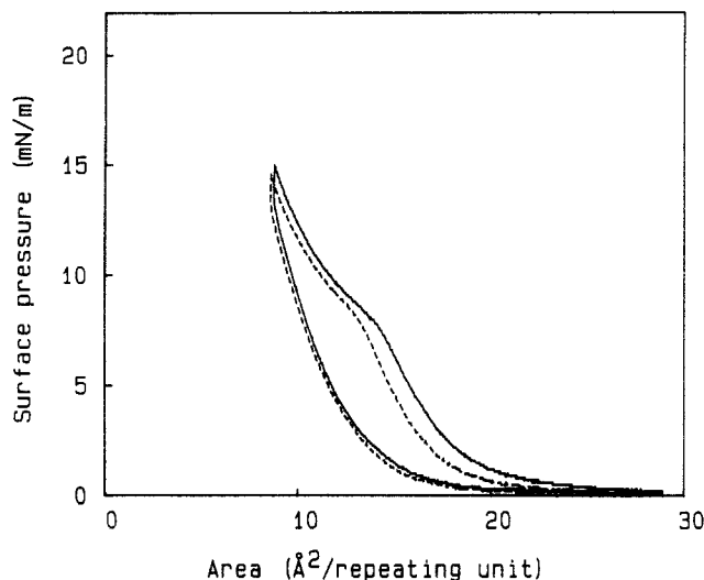
Figure 5. Hysteresis isotherms of stereoblock PMMA, T = 45 °C, compression and decompression speed 2 \text{ \AA}^2/(\text{mmu}\cdot\text{min}) . The solid line represents the first cycle, and the dashed line represents the second cycle.
