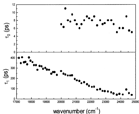
Fig. 6. Energy dependence of epar-me decay times.
