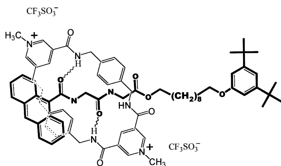
Fig. 1. Schematized chemical structure of epar-me. The thread is drawn using bold bonds, hydrogen bonds are drawn as “wavy” bonds.
