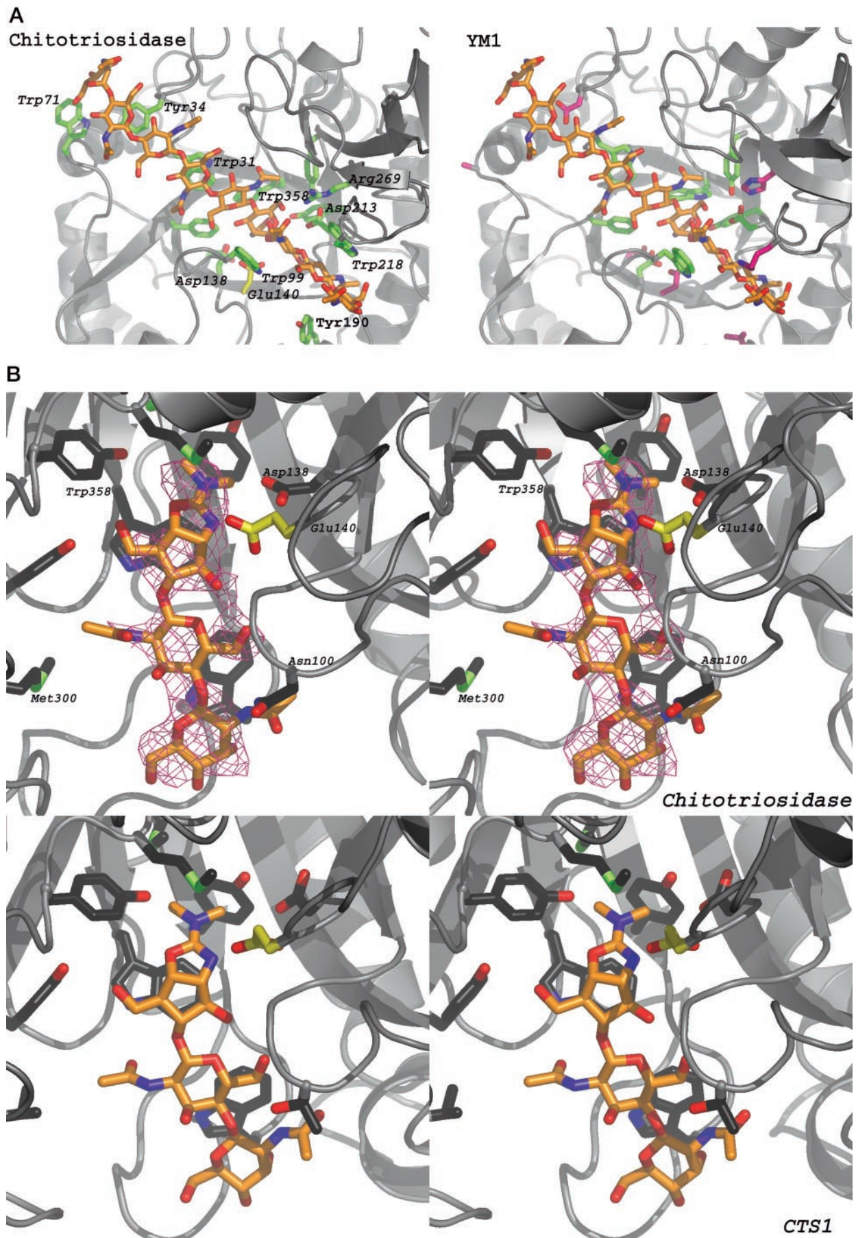
FIG. 3. Comparison of active site details and interaction with allosamidin. In A, the substrate binding pockets of the human chitotriosidase and YM1 are compared. Protein backbones are represented by a gray ribbon . A model of NAG 9 , in equivalent position to that in Fig. 1, is
