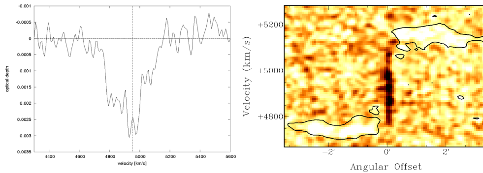
Fig. 2. B2 0259+35: Left panel: H I absorption against the unresolved nucleus as derived from the new WSRT observations (Struve et al. in prep.). The total absorption width is larger than 400 \text{ km s}^{-1} . The vertical line indicates the systemic velocity. Right panel: Position-velocity plot of the H I (grey-scale and contours) taken along the major axis (PA = 75^\circ ).
