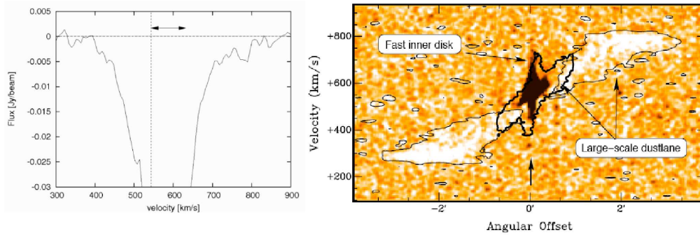
Fig. 1. Centaurus A: Left panel: H I absorption against the unresolved nucleus as derived from the ATCA observations (Morganti et al. 2008). The total absorption width ranges from 400 to 800 km s -1 . The arrow indicates the previously known (redshifted) absorption. The vertical line gives the systemic velocity. Right panel: Position-velocity plot of the H I (grey-scale and thin contours) and superimposed the CO emission (thick contours; from Liszt (2001), taken along position angle 139°). Note that the CO observations do not extend beyond a radius of about 1 arcmin. Figure taken from Morganti et al. (2008).
