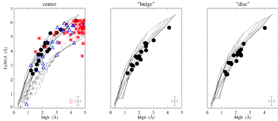
Figure 2. Index-index plots of Fe 5015 against Mg b, showing the [Mg/Fe] abundance ratios in the centres of the galaxies. Symbols as in Figure 1. Shown are model grids for single age-metallicity stellar populations, from Thomas et al. (2003), for [Mg/Fe]=0 (full lines) and [Mg/Fe]=0.5 (dashed lines). One sees that [Mg/Fe] for the late-type spirals is consistent with solar values. Plotted are the central line indices on the left, the bulge in the middle, and the disk, as covered by the SAURON field, on the right.
