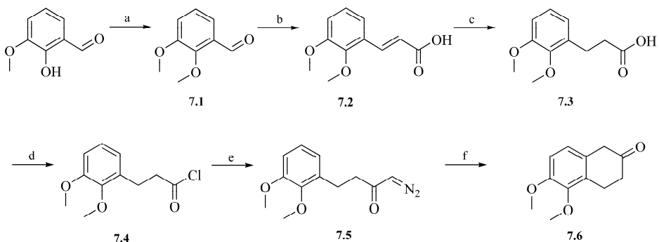
Scheme 7.2 Synthesis of 5,6-dimethoxy-2-tetralone ( 7.6 ) according to Copinga et al. Reagents and conditions: a) \text{K}_2\text{CO}_3 , (\text{CH}_3)_2\text{SO}_4 , MeOH, reflux, overnight; b) malonic acid, piperidine, pyridine, 75^\circ\text{C} , 2h, reflux, overnight; c) 3.5 bar \text{H}_2 , 10% Pd/C, 96% EtOH, RT; d) \text{SOCl}_2 , toluene, reflux, 1h; e) diazomethane, \text{Et}_2\text{O} , 5^\circ\text{C} , RT, overnight; f) [\text{Rh}(\text{CH}_3\text{COO})_2]_2 , \text{CH}_2\text{Cl}_2 , reflux for 20 min, \text{CF}_3\text{COOH} , 15 min reflux.
