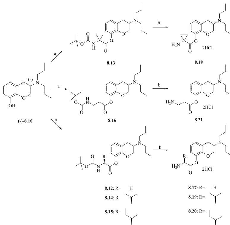
Scheme 8.4 Synthesis of glycine ( 8.17 ), 1-aminocyclopropane-1-carboxylic acid ( 8.18 ), L-valine ( 8.19 ), L-isoleucine ( 8.20 ) and \beta -alanine ( 8.21 ) (-)-3,4-dihydro-3-( N,N -di- n -propylamino)-2 H -1-benzopyran-8-yl esters as 2HCl salts. Reagents and conditions: a) EDC, N - tert -Boc-amino acid, HOBt hydrate, 0°C-RT; b) 4N HCl in dioxane, RT.
