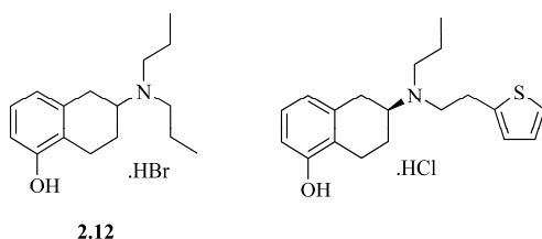
Figure 2.1 Structures of 5-OH-DPAT.HBr and rotigotine.HCl.
