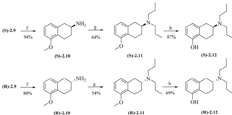
Scheme 2.2 Synthesis of ( S )-5-OH-DPAT (( S )- 2.12 ) and ( R )-5-OH-DPAT (( R )- 2.12 ). Reagents and conditions: f) 3.5 bar H 2 , 10% Pd/C in EtOH, 40 °C; g) 1-iodopropane (4 eq), K 2 CO 3 in acetonitrile, reflux; h) 48% HBr, reflux.
