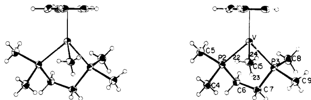
Figure 3. ORTEP stereo drawing of \text{CpVCH}_3(\text{dmpe}) showing atom labeling. Cyclopentadienyl carbons are C(10) through C(14). Methyl hydrogens only are indicated by small numbers.
