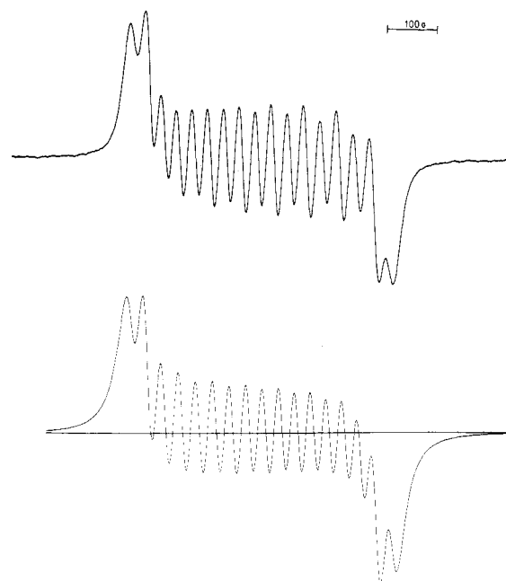
Figure 2. (a) EPR spectrum of CpV(BH 4 )dmpe in toluene solution at 25 °C (above) and (b) calculated spectrum (below).
