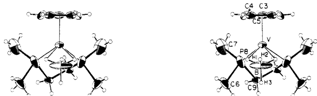
Figure 4. ORTEP stereo drawing of \text{CpV}(\text{BH}_3)\text{dmpe} showing atom labeling. C(3), V, B, H(2), and H(3) lie on a crystallographic mirror plane.
