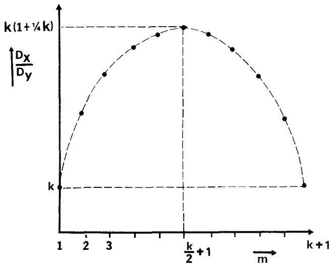
Fig. 5. Ratio of the diffusion coefficients in the horizontal and vertical direction as a function of the position m of shifted bonds.
