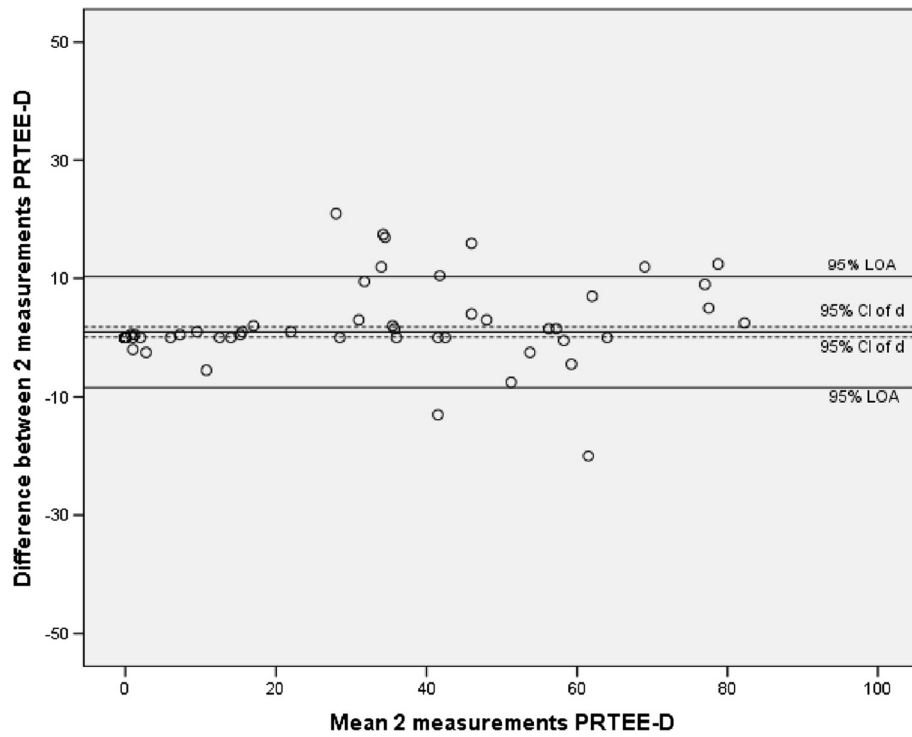
Figure 1 Bland and Altman plot of reliability (agreement) of the PRTEE-D (2 measures).
