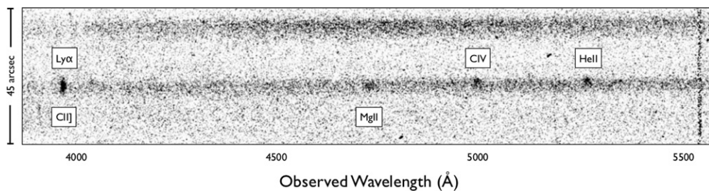
Figure 4. Negative image of the blue side of the Keck LRIS spectrum of 3C 220.3. The horizontal and vertical axes represent the spectral and spatial dimensions, respectively. The horizontal dark stripe in the middle of the frame corresponds to the 3C 220.3 system, and the upper dark stripe originates from the faint extended source labeled “ser 1” in Figure 2. The 3C 220.3 stripe has a width of \sim 4'' , the lower part originating from source B, the central part from source A, and the upper part from the arc. The dark knots in the stripe are due to emission lines as labeled. Mg II \lambda 2798 from the radio galaxy (source A) is centrally located in the continuum, while the C IV and He II lines are offset upward, indicating an origin in the arc. The line on the left side (at 3920 \text{ \AA} ) seems more central, suggesting it is primarily C II from the radio galaxy rather than Ly \alpha from the lensed SMG.
