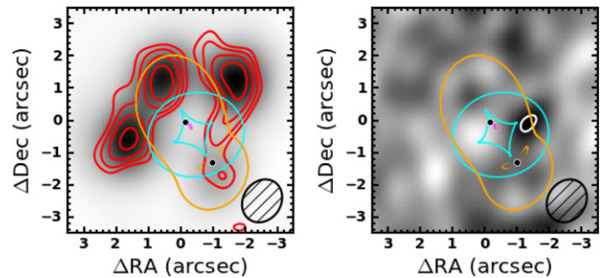
Figure 12. Left: SMA imaging (red contours, starting at 2\sigma and increasing by factors of 1.4) overlaid on the inverted, deconvolved map of the best-fit model visibilities (gray scale). The critical curve and caustics are represented by solid orange and cyan lines, respectively. The position of the lenses and the source are shown by plus signs and a magenta filled ellipse, respectively. The FWHM of the synthesized beam is shown in the lower right corner of each panel. Right: residual image (gray scale) obtained by inverting and deconvolving the residual visibilities (i.e., the difference between the model and data visibilities). Black and white contours indicate \pm 2\sigma level. A 2\sigma peak in the map of the residual visibilities may be an indication of additional minor structures in the lens plane or in the source plane.
