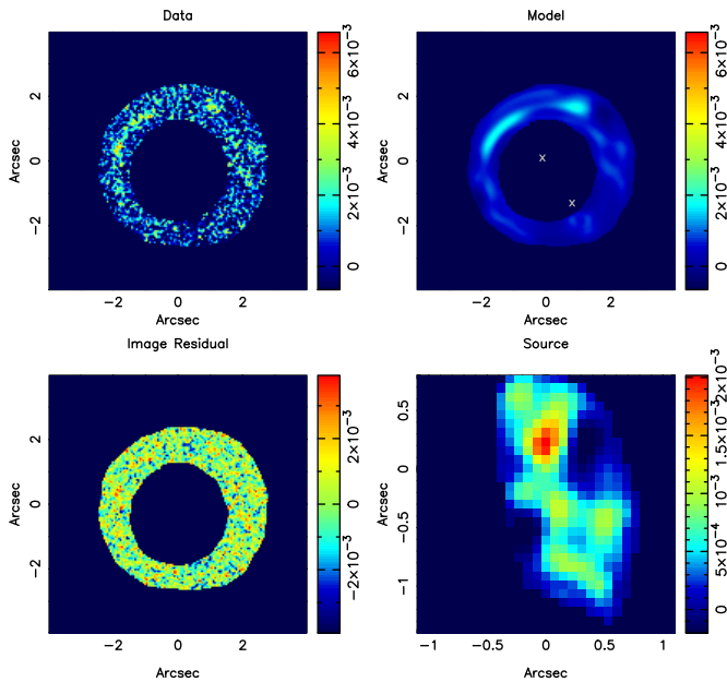
Figure 11. Results from modeling the HST 702 nm image with the double lens model derived from the Keck AO image. The area other than the Einstein ring is masked out. North is up and east is to the left. Top left: data after subtraction of A and B. Top right: modeled image. The crosses mark the positions of A and B. Bottom left: residual image, data minus model image. Bottom right: reconstructed image of the source in the source plane.
