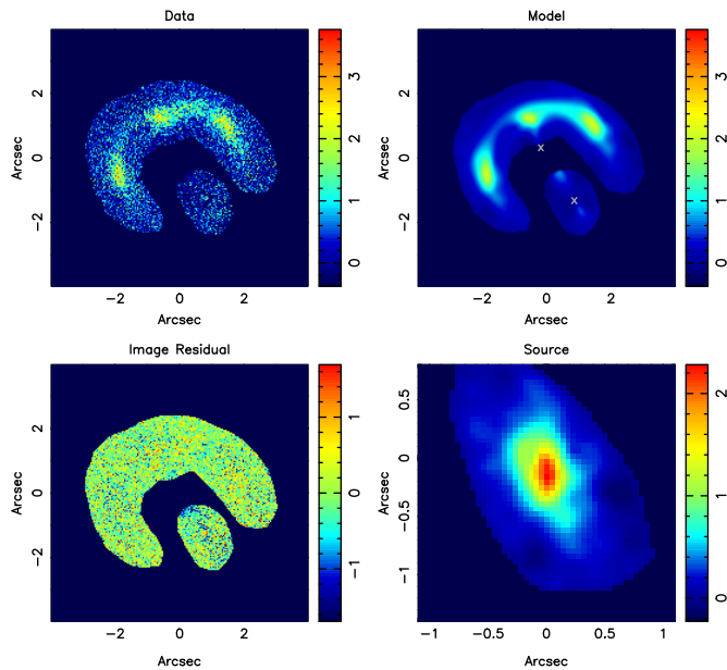
Figure 9. Results from modeling the Keck AO image with a double lens. The regions outside the Einstein half ring and source B are masked and not used for the model fit. North is up and east is to the left. Top left: data after subtraction of A and B. Top right: modeled image. The crosses mark the positions of A and B. There are two very faint objects, one between A and B and one southwest of B; they may be the central image and the counter-image of the arc. Bottom left: residual image, data minus model image. Bottom right: reconstructed image of the source in the source plane.
