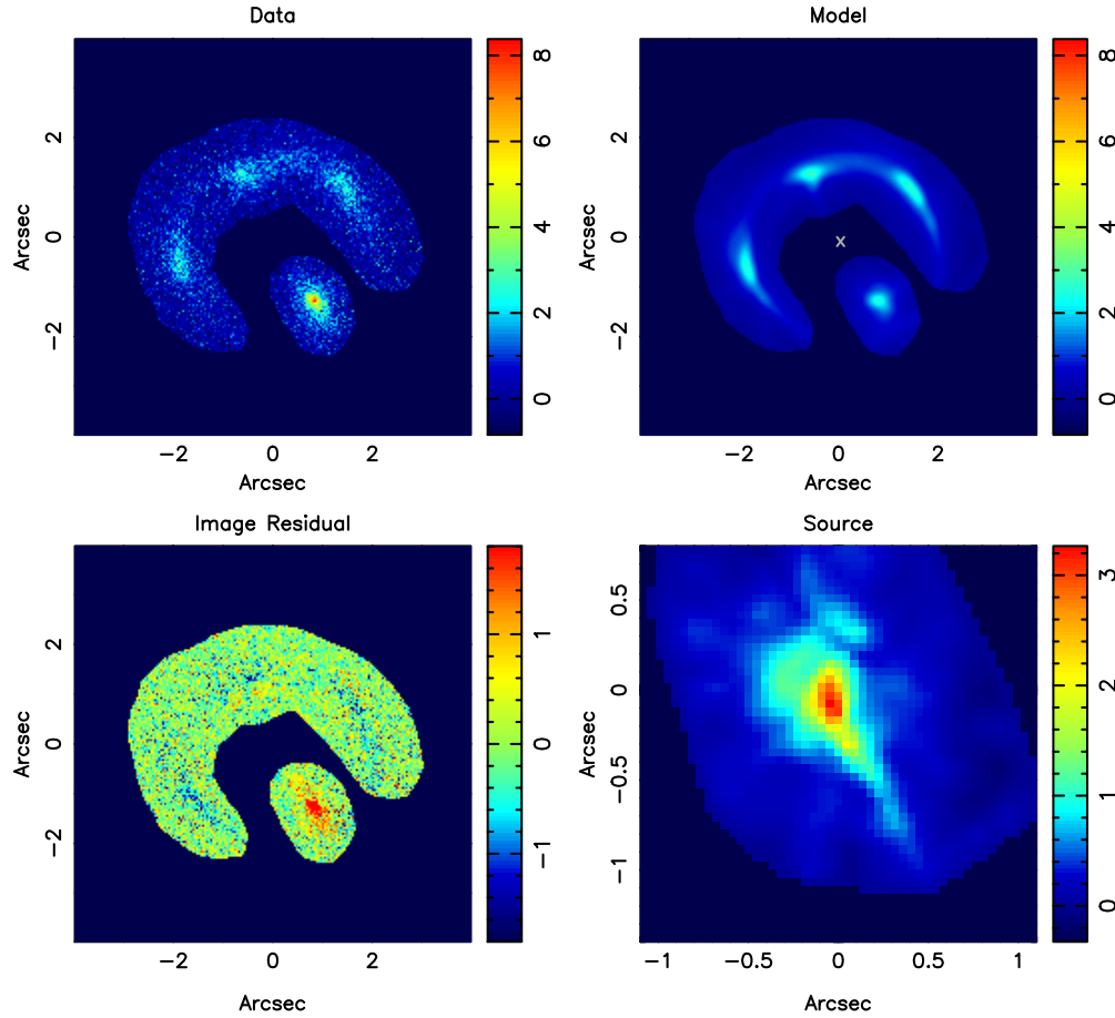
Figure 7. Results from modeling the Keck AO image with a single lens centered on galaxy A, located at (0, 0). The regions outside the Einstein half ring and source B are masked and not used for the model fit. While the total map has 200 \times 200 = 40,000 pixels, the area used for modeling has 10,912 pixels. North is up and east is to the left. Top left: data after subtraction of A. Top right: modeled image. The cross marks the position of A. Bottom left: residual image, data minus model image. Bottom right: reconstructed image of the source in the source plane ( 50 \times 50 = 2500 source pixels).
