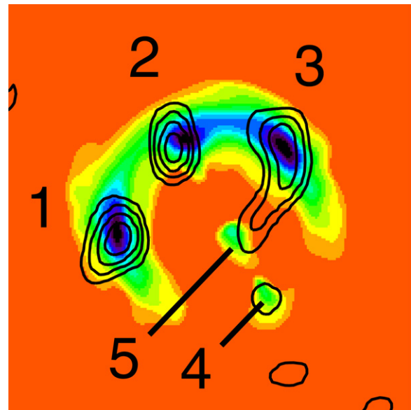
Figure 10. Modeled Keck AO image (color representing surface brightness) based on the double lens. Frame size is 7''.5 . Superposed contours show the SMA map with the three bright knots labeled. The contours start at 2.5\sigma and increase in steps of 1\sigma . Source image 4 coincides with a faint 1 mm contour. Source image 5 could be indicated by the faint tail of knot 3. Galaxy B lies between knots 4 and 5.
