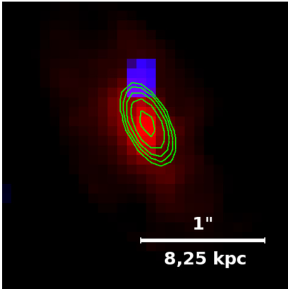
Figure 13. Source image of the SMG reconstructed from the Keck, HST , and SMA images. The stellar emission (Keck \sim 680 nm restframe) is shown in red, UV ( HST \sim 218 nm restframe) in blue, and the dust emission (SMA \sim 310 \mu\text{m} restframe) as green contours (logarithmic). North is up and east is to the left.
