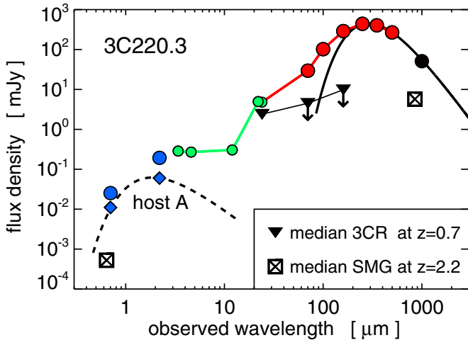
Figure 6. Spectral energy distribution of the 3C 220.3 system. Filled circles show flux densities from the entire source: large red ( Herschel ), small green ( WISE and Spitzer ), large black ( SMA ), large blue ( HST and Keck ). A solid line shows a graybody fit through the SMA and \geq 250 \mu\text{m} Herschel data points ( T = 36 \text{ K} at z = 2.221 , dust emissivity index \beta = 1.5 ). Blue diamonds show the HST and Keck flux densities of lens A (defined in Figure 1) connected by a blackbody (dashed line). Triangles show the median 24–160 \mu\text{m} flux densities of twelve 3C radio galaxies at z \sim 0.7 . X-squares show the median R -band and 850 \mu\text{m} flux densities of 73 SMGs at z \sim 2.2 (Chapman et al. 2005).
