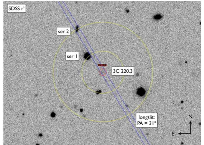
Figure 2. Keck LRIS slit position (blue lines) overlaid on an SDSS r -band negative image of the 3C 220.3 system. The small red circle marks the location of 3C 220.3, and the larger yellow circles (radii 19'' and 45'' ) go through two serendipitously hit sources labeled “ser 1” and “ser 2.”
