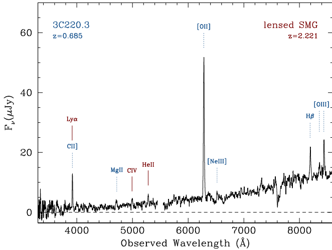
Figure 3. Keck LRIS spectrum of 3C 220.3 system with prominent lines labeled. Blue dotted lines label emission lines associated with the radio galaxy at z = 0.685 , while red solid lines label emission lines associated with the lensed SMG at z = 2.221 . The feature at 3921 \text{ \AA} is associated with emission lines from both sources. The gap at 5500 \text{ \AA} corresponds to the dichroic separating the blue and red arms of LRIS. Absorption at 7600 \text{ \AA} is due to the uncorrected atmospheric A band.
