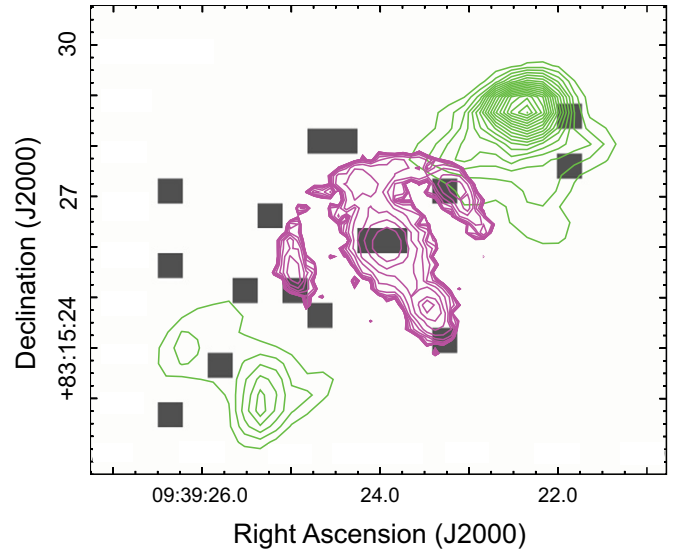
Figure 5. Chandra X-ray photon image (black squares) toward 3C 220.3, with Keck K' -band contours (violet) and 6 cm radio contours (green; from Mullin et al. 2006).
