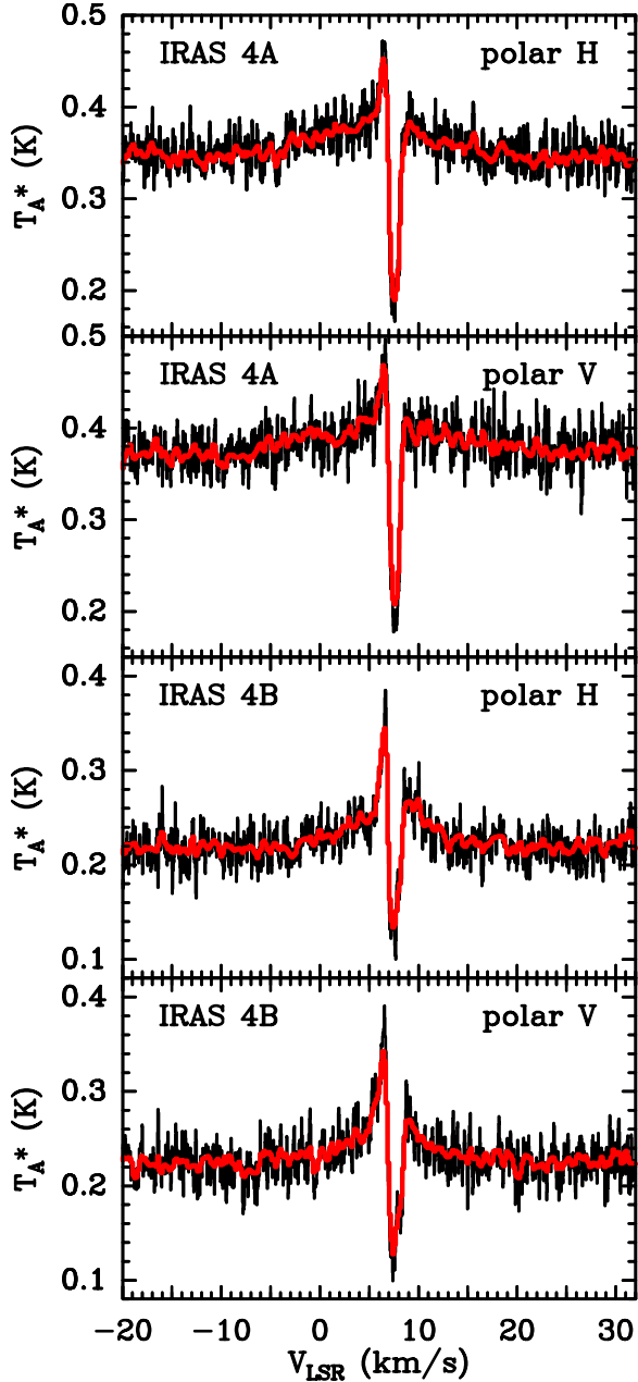
Fig. A.1. Comparison of the WBS (red) and HRS (black) spectra obtained at 894 GHz with Herschel /HIFI towards IRAS 4A and IRAS 4B for the H and V polarizations.
