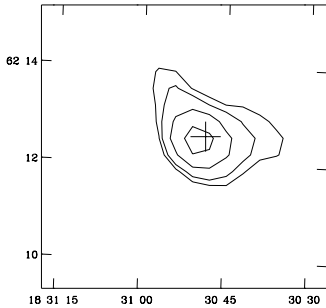
WNB1830+6212 S *
