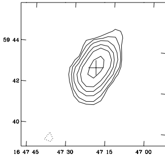
WNB1647+5942 S *
