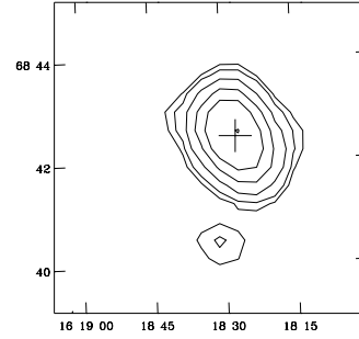
WNB1618+6842 S
