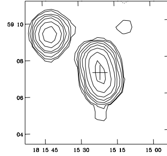
WNB1815+5907 S
