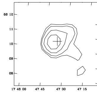
WNB1747+6810 S *
