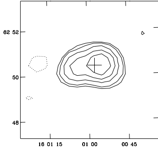
WNB1600+6250 S
