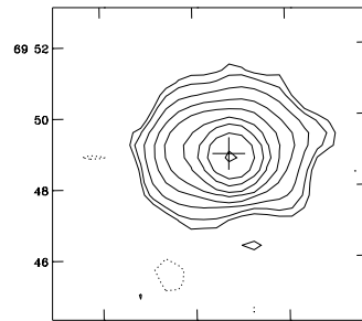
WNB1807+6948 S *
