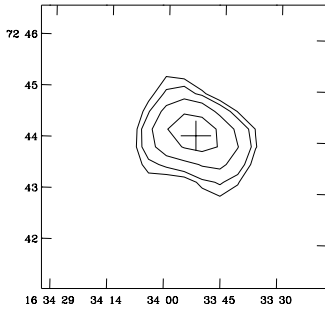
WNB1633+7244 S
