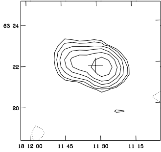
WNB1811+6321 S
