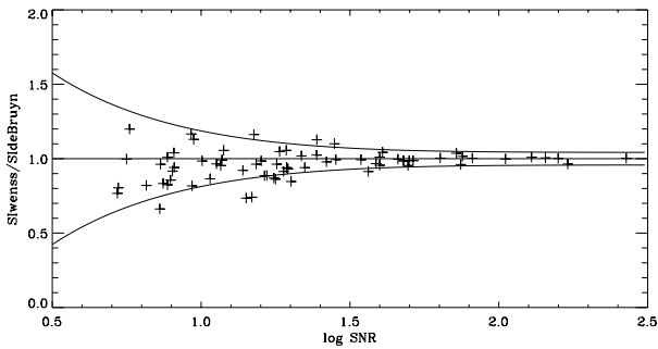
Fig. 8. The ratio of integrated flux densities as measured by WENSS ( SI_{wenss} ) and a standard WSRT observation ( SI_{deBruyn} ), as a function of the signal-to-noise ratio in WENSS. The curves represent 1\sigma errors, under the assumption that the error in the standard WENSS observation is comparable to the error in the WENSS data
