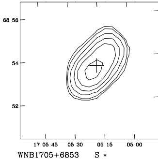
WNB1705+6853 S *
