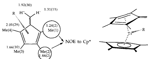
Fig. 1. (a) NMR characteristics and (b) structure in solution of Cp* FvTiR.
