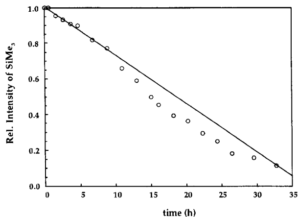
Fig. 2. Decomposition of \text{Cp}^* \text{FvTiCH}_2\text{SiMe}_3 at 381 K in benzene- d_6 as monitored by ^1\text{H} NMR, showing the relative intensity of the trimethylsilyl signal, and an extrapolated linear fit to the first six data points.
