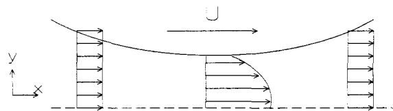
Figure 10. Flow profile in the calender gap.
