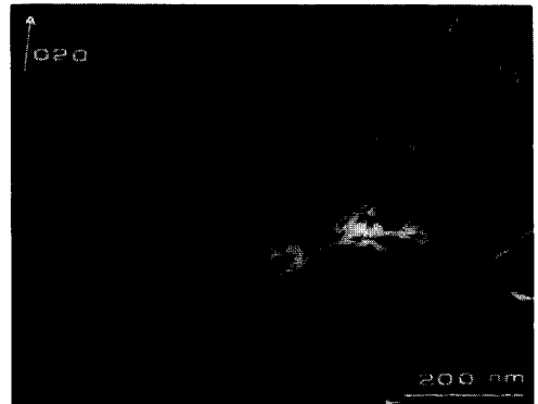
Fig. 5 (Left) Slip-bands with a pile-up of dislocations bound at a cell boundary. Fig. 6 (Right) Pile-up of dislocations near a cell boundary.
