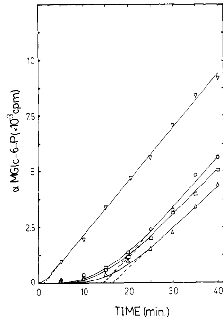
FIGURE 5: Phosphorylation of \alpha -MeGlc as a function of time and preincubation. The following components were preincubated: ( \circ ) none, ( \Delta ) E_I plus Mg^{2+} (2.5 mM), ( \square ) E_I plus PEP (5.0 mM), ( \nabla ) E_I plus Mg^{2+} (2.5 mM) plus PEP (5.0 mM). The preincubation was carried out as described under Materials and Methods.
