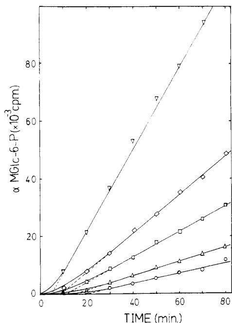
FIGURE 1: Phosphorylation of \alpha -MeGlc as a function of time and E_I concentration. The E_I concentrations are ( \circ ) 0.25, ( \Delta ) 0.38, ( \square ) 0.50, ( \diamond ) 0.63, and ( \nabla ) 1.25. E_{II} (20 \mu L) was added as a membrane suspension, prepared as described under Materials and Methods.
