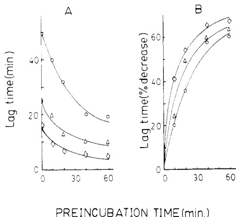
FIGURE 7: (A) Lag time as a function of the length of the preincubation of E 1 , PEP, and Mg 2+ at rate-limiting amounts of E 1 (μg/mL): (O) 0.13, (Δ) 0.25, (◇) 0.50. (B) Relative decrease of the lag time obtained from the data in (A). Percent decrease = [1 - \text{LT}(t)/\text{LT}(t = 0)] \times 100 , where LT( t ) is the lag time after preincubation time t .
