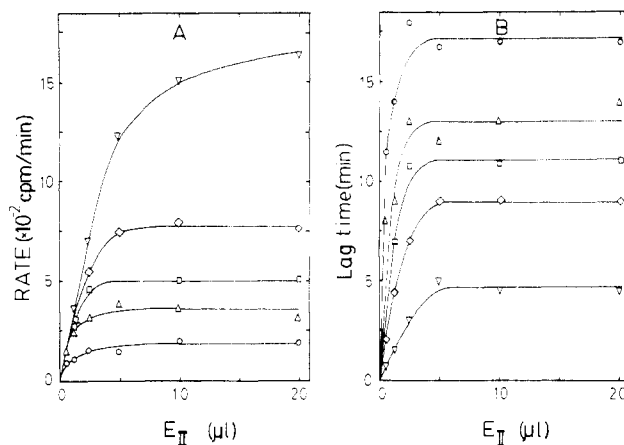
FIGURE 3: Rates of phosphorylation (A) and lag times (B) as a function of the E_{II} concentration at several E_I concentrations ( \mu g/mL): ( \circ ) 0.25, ( \Delta ) 0.38, ( \square ) 0.50, ( \diamond ) 0.63, ( \nabla ) 1.25. The determination of the rates and the lag times from the time curves, as presented in Figures 1 and 2, is described in the text.
